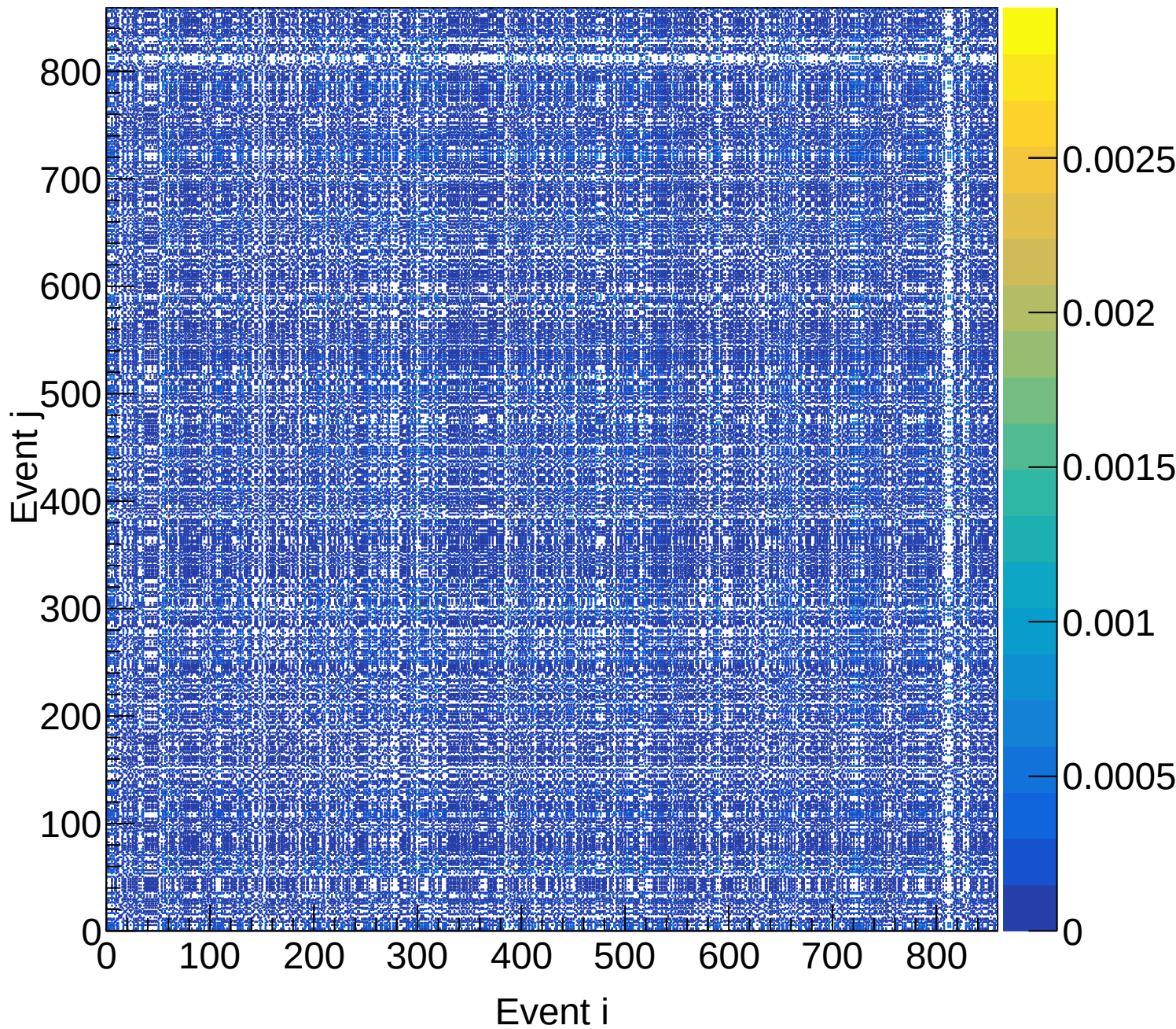
LH2 (total) Covariance | M: [3.9, 4.2) xF: [0.40, 0.45)
