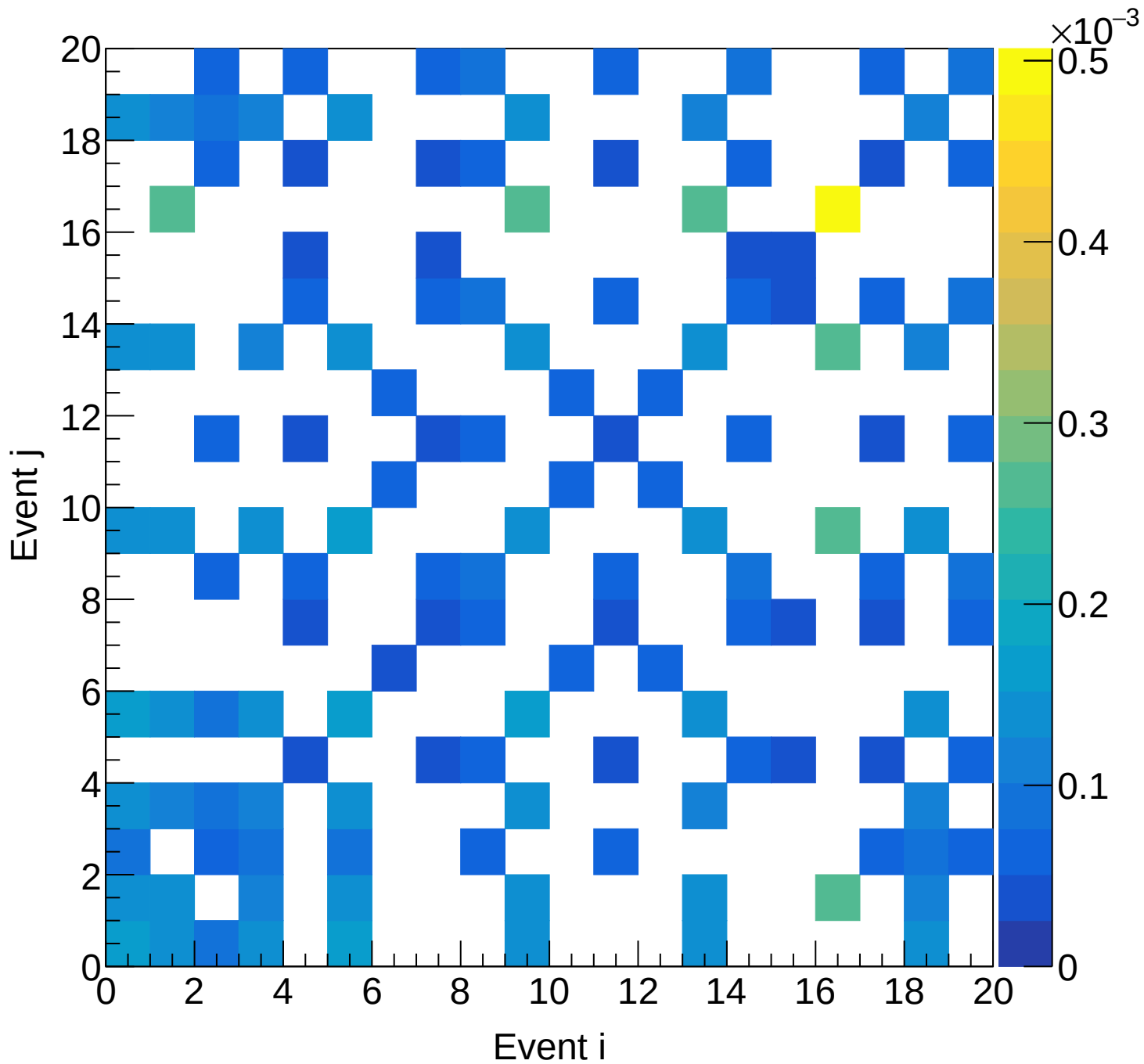
LH2 (total) Covariance | M: [6.9, 7.5) xF: [0.40, 0.45)
