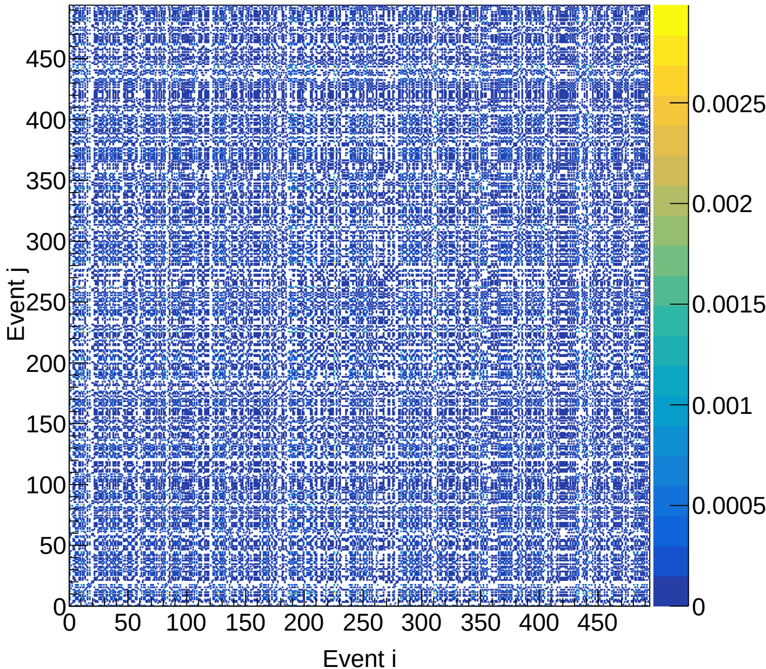
LH2 (total) Covariance | M: [4.5, 4.8) xF: [0.40, 0.45)
