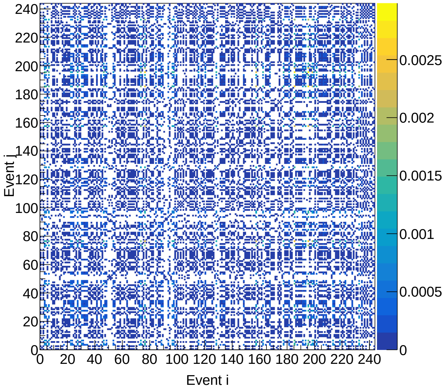
LH2 (total) Covariance | M: [5.1, 5.4) xF: [0.40, 0.45)
