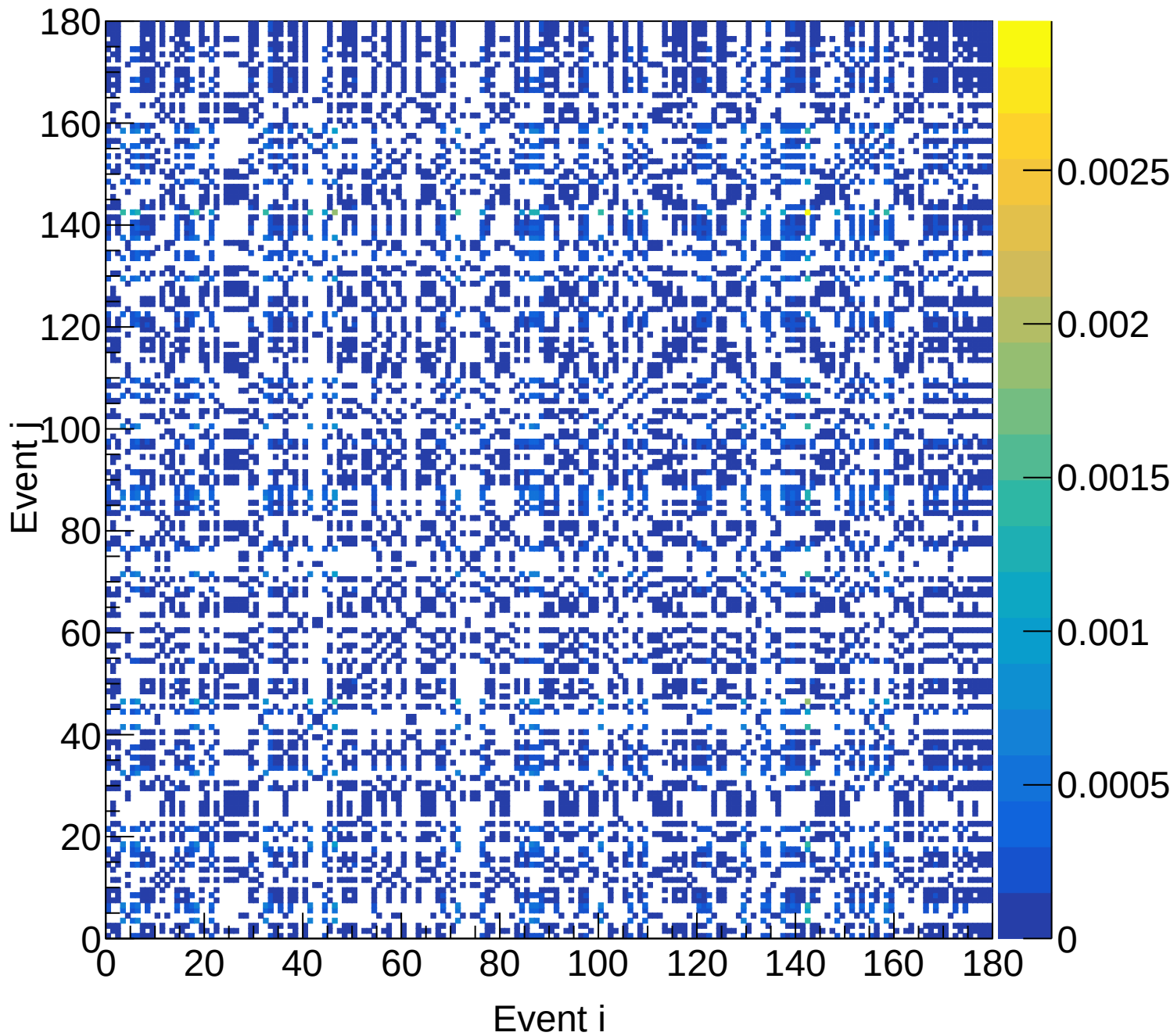
LH2 (total) Covariance | M: [5.4, 5.7] xF: [0.40, 0.45)
