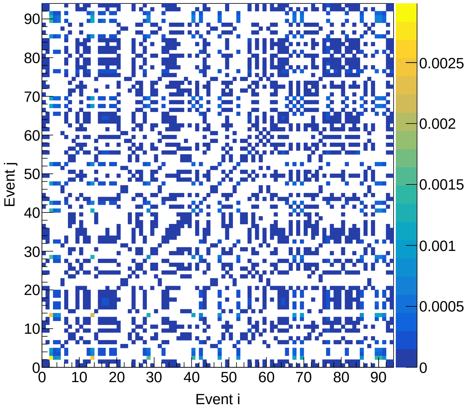
LH2 (total) Covariance | M: [5.7, 6.0] xF: [0.40, 0.45)
