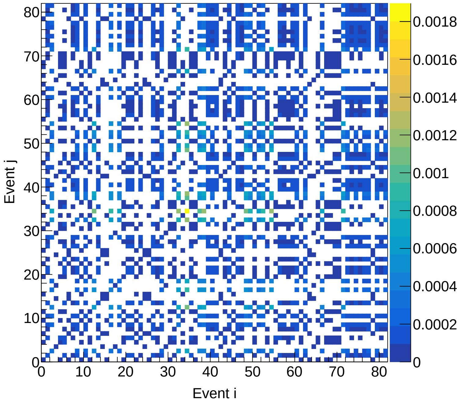
LH2 (total) Covariance | M: [6.0, 6.3) xF: [0.40, 0.45)
