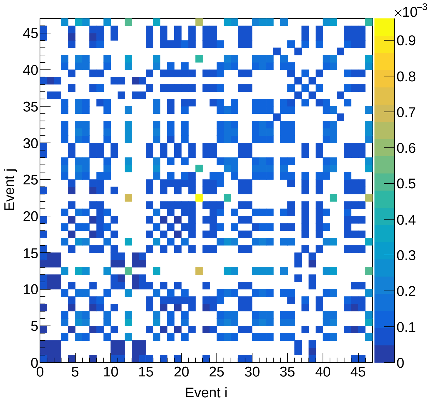
LH2 (total) Covariance | M: [6.3, 6.6) xF: [0.40, 0.45)
