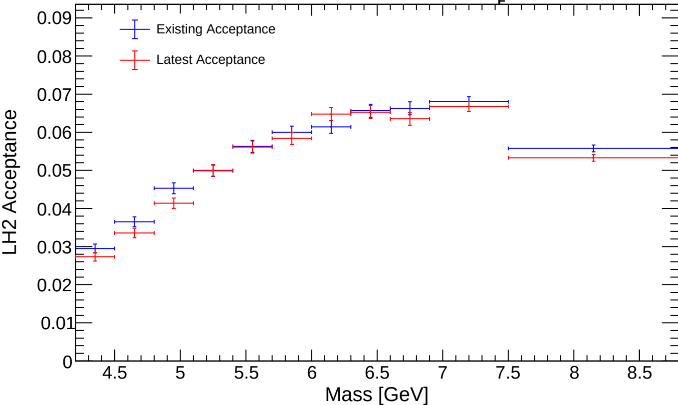
LH2 Existing vs Latest: Mass in x_E Bin 12
