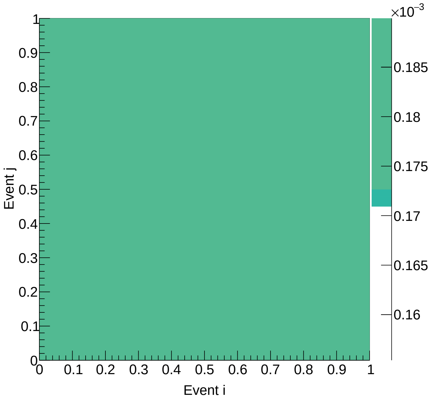
Flask (mix) Covariance | M: [5.1, 5.4) xF: [-0.05, 0.00)
