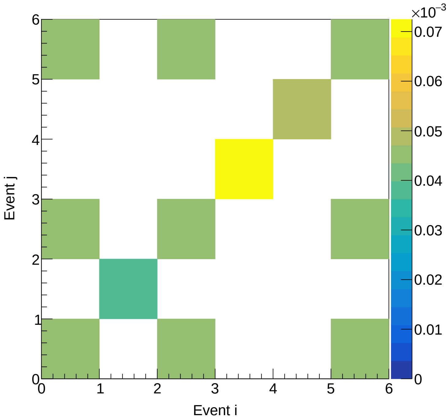
Flask (mix) Covariance | M: [3.9, 4.2) xF: [0.50, 0.55)
