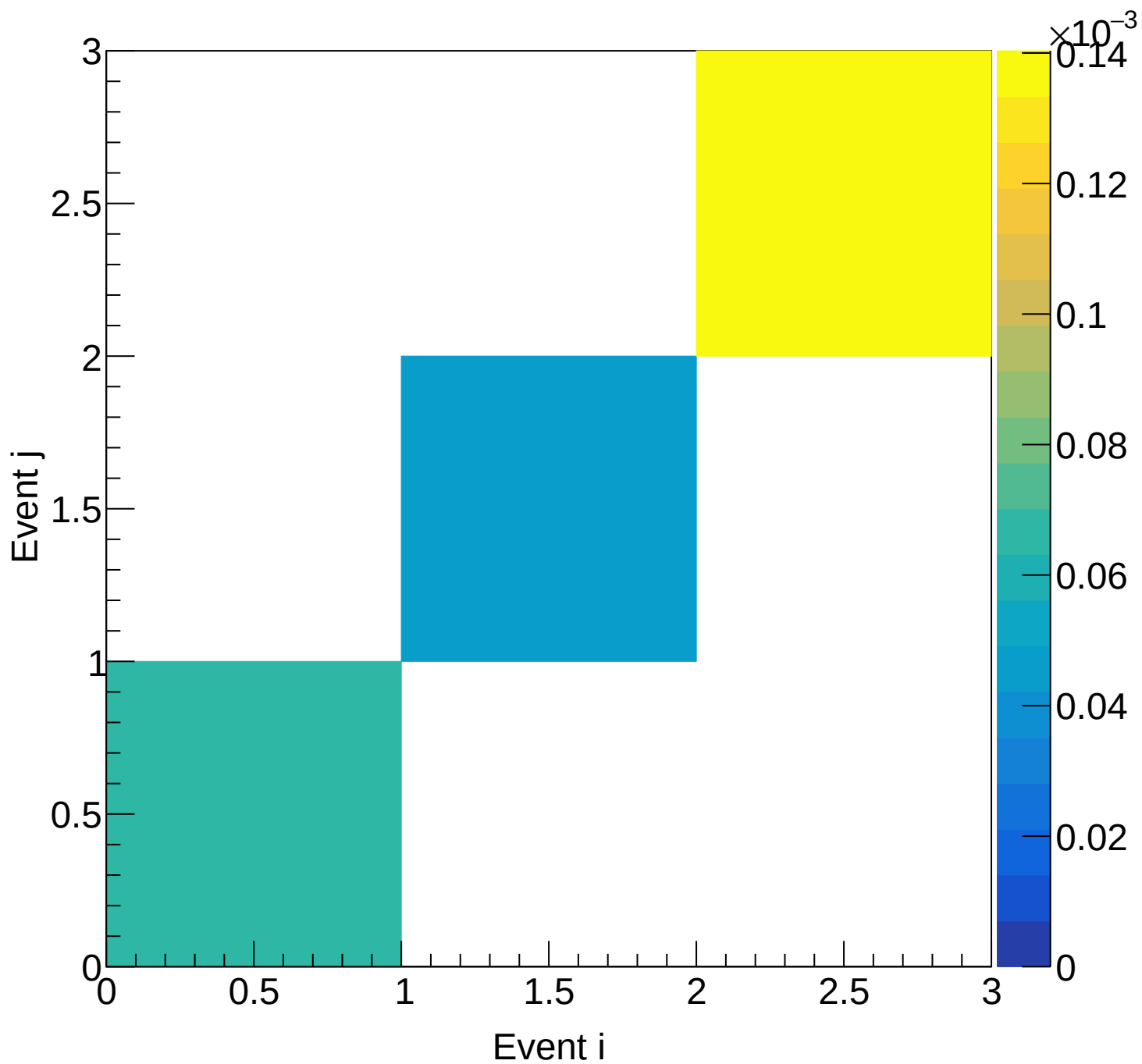
Flask (mix) Covariance | M: [4.2, 4.5) xF: [0.50, 0.55)
