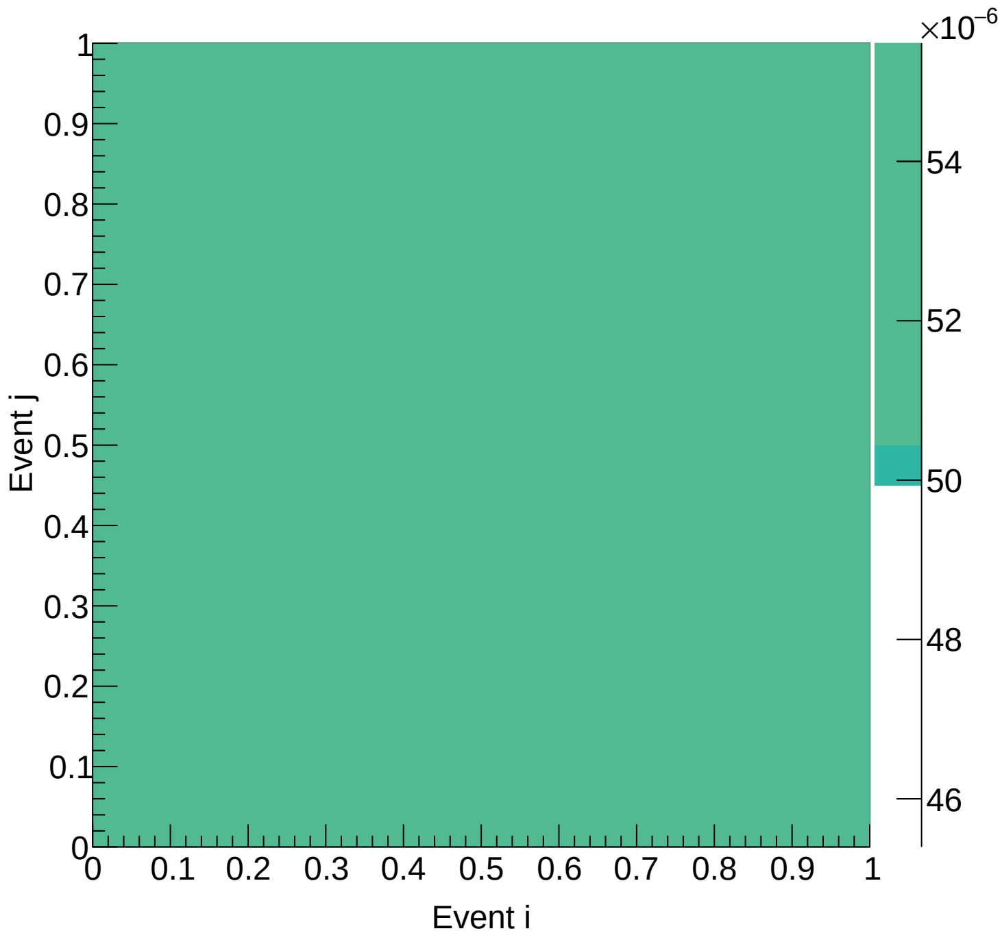
Flask (mix) Covariance | M: [4.5, 4.8) xF: [0.60, 0.65)
