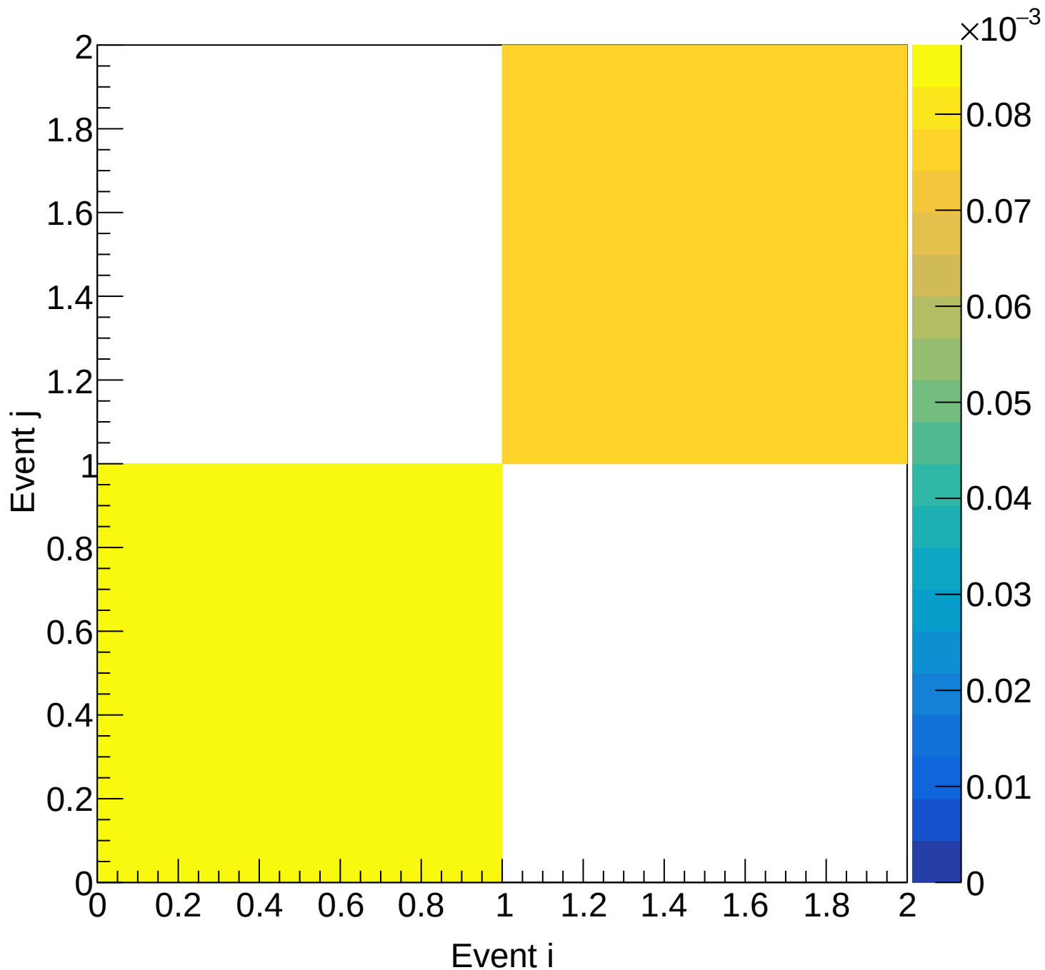
Flask (mix) Covariance | M: [4.2, 4.5) xF: [0.75, 0.80)
