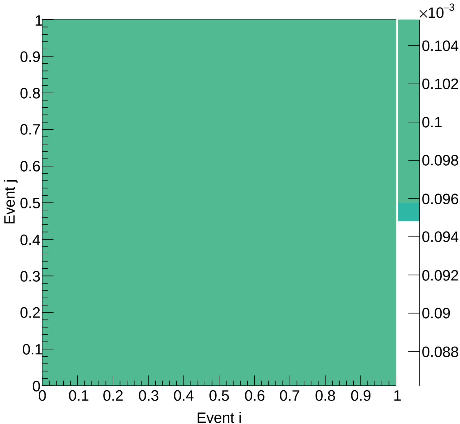
Flask (mix) Covariance | M: [3.9, 4.2) xF: [0.80, 0.85)
