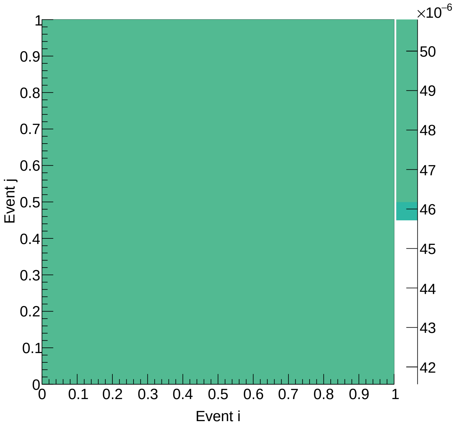
Flask (mix) Covariance | M: [5.4, 5.7) xF: [0.00, 0.05)
