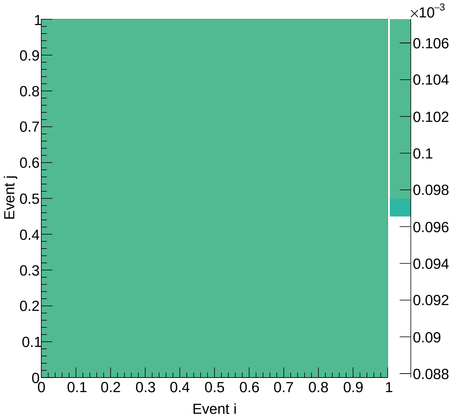
Flask (mix) Covariance | M: [5.1, 5.4) xF: [0.05, 0.10)
