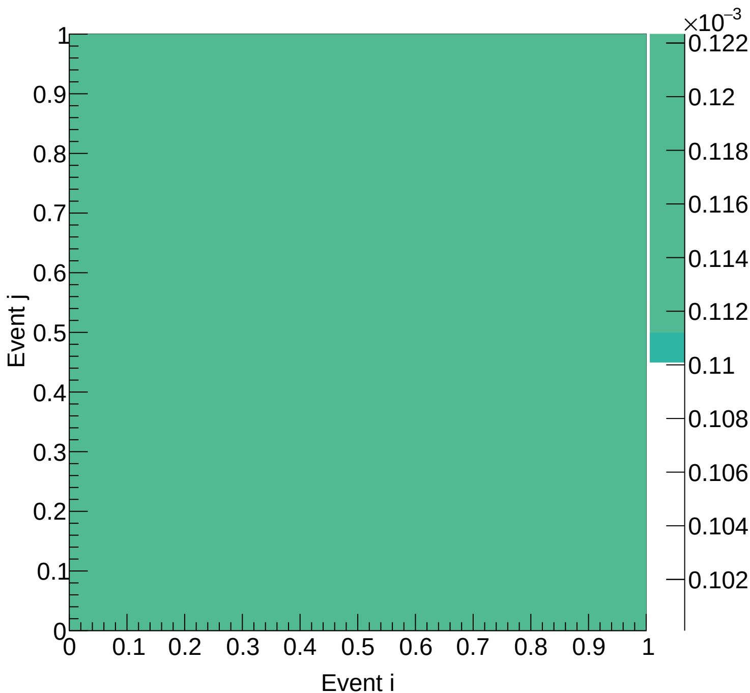
Flask (mix) Covariance | M: [6.0, 6.3) xF: [0.05, 0.10)
