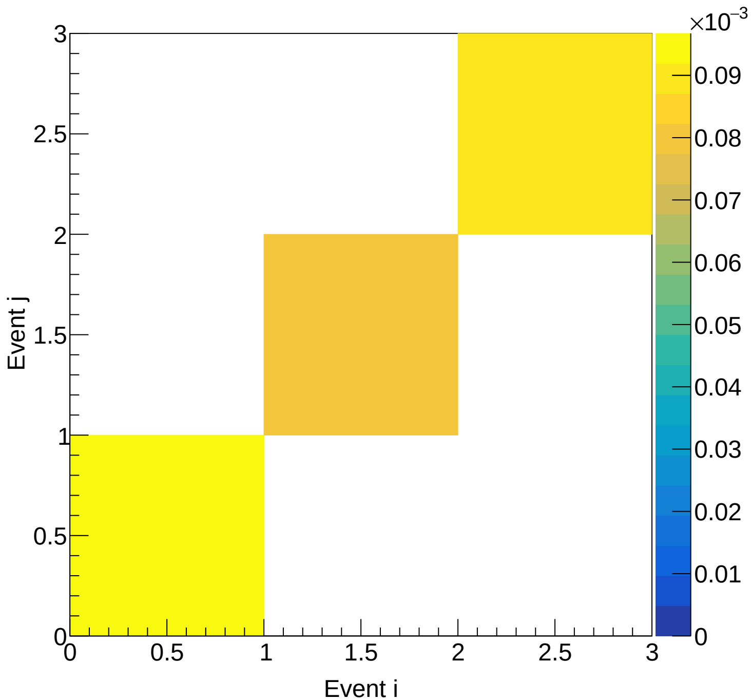
Flask (mix) Covariance | M: [4.8, 5.1) xF: [0.10, 0.15)
