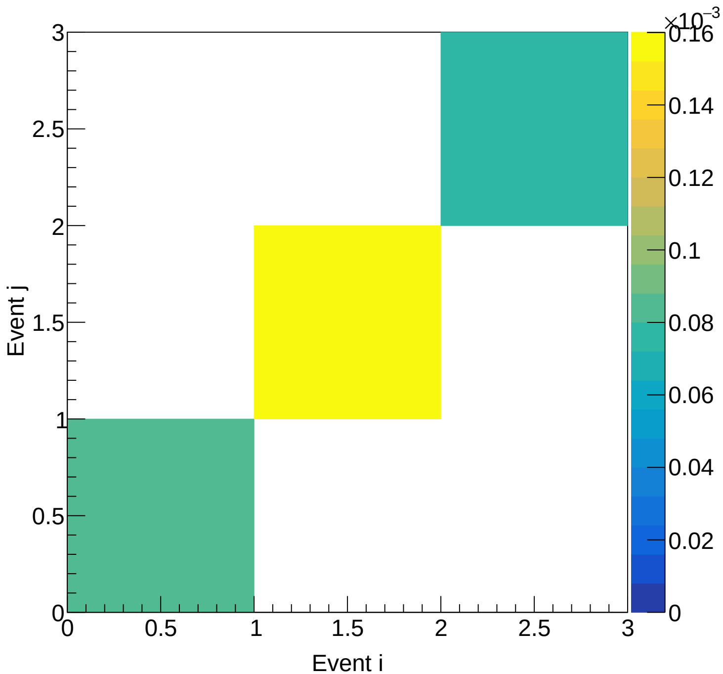
Flask (mix) Covariance | M: [4.2, 4.5) xF: [0.15, 0.20)
