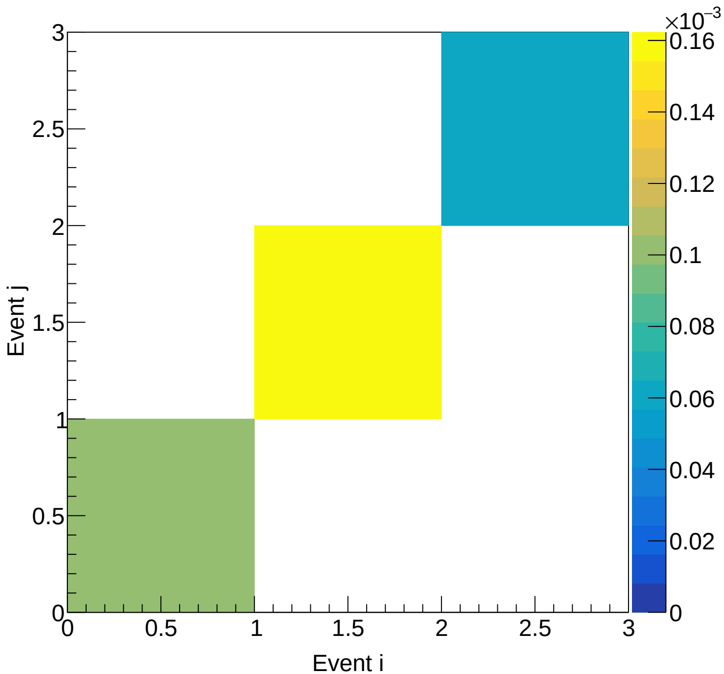
Flask (mix) Covariance | M: [5.4, 5.7) xF: [0.15, 0.20)
