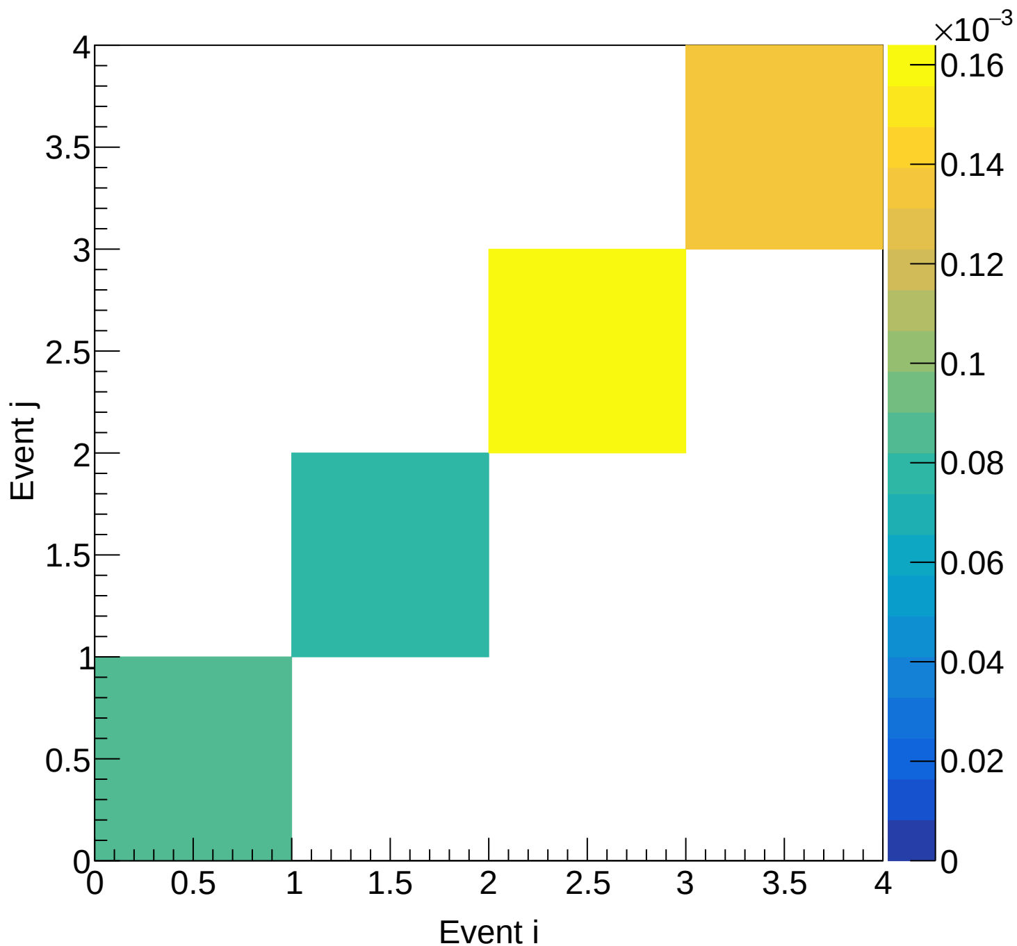
Flask (mix) Covariance | M: [4.2, 4.5) xF: [0.20, 0.25)
