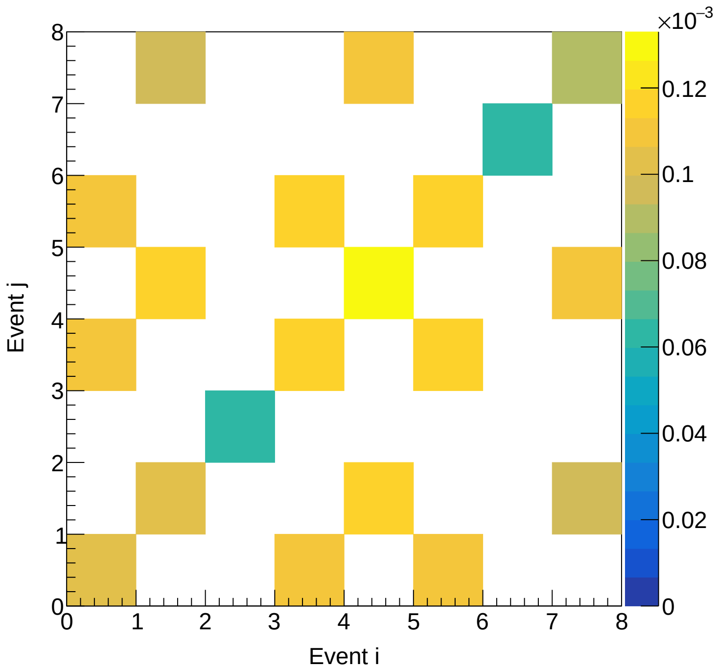
Flask (mix) Covariance | M: [4.8, 5.1) xF: [0.20, 0.25)
