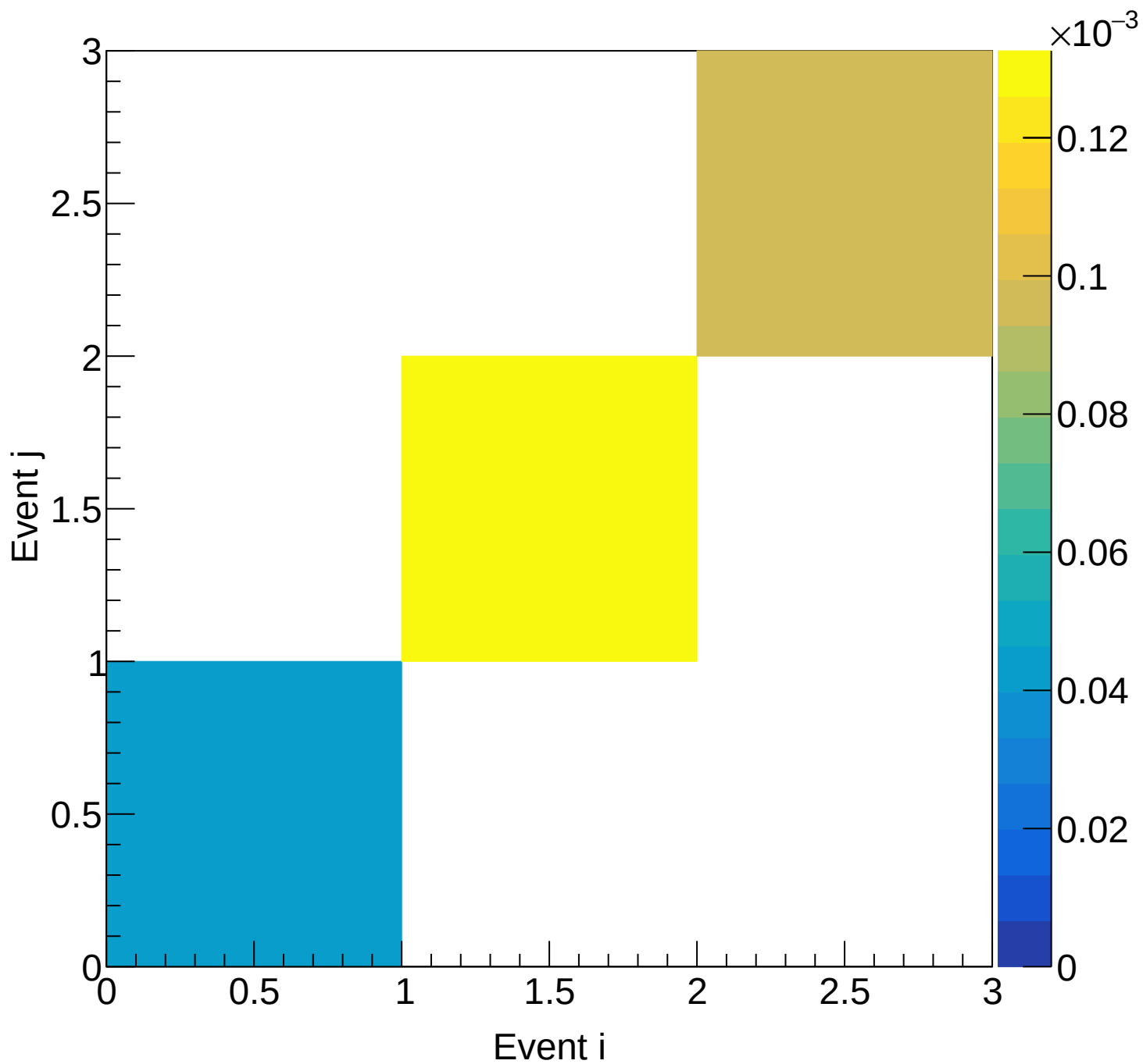
Flask (mix) Covariance | M: [4.2, 4.5) xF: [0.25, 0.30)
