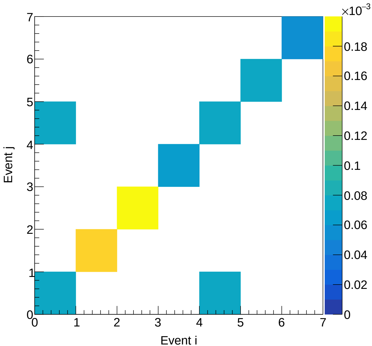
Flask (mix) Covariance | M: [4.5, 4.8) xF: [0.25, 0.30)
