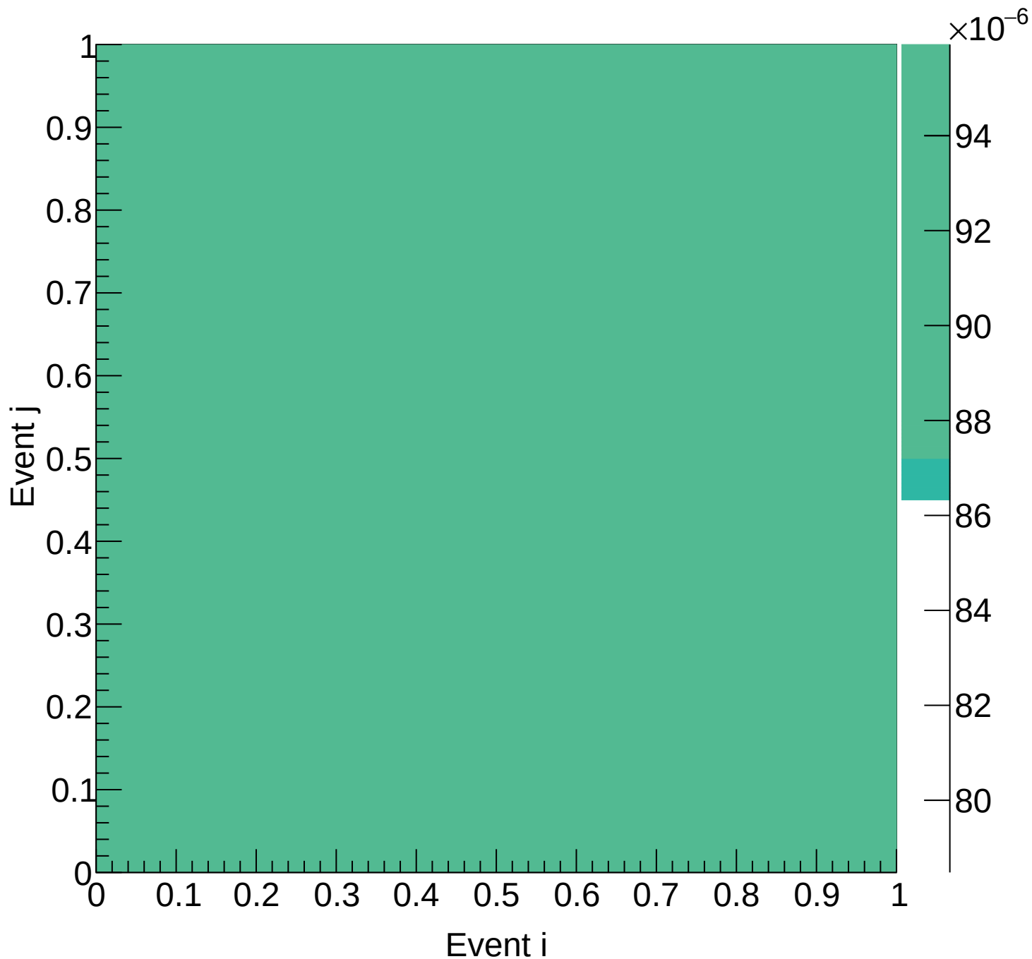
Flask (mix) Covariance | M: [5.4, 5.7) xF: [0.25, 0.30)
