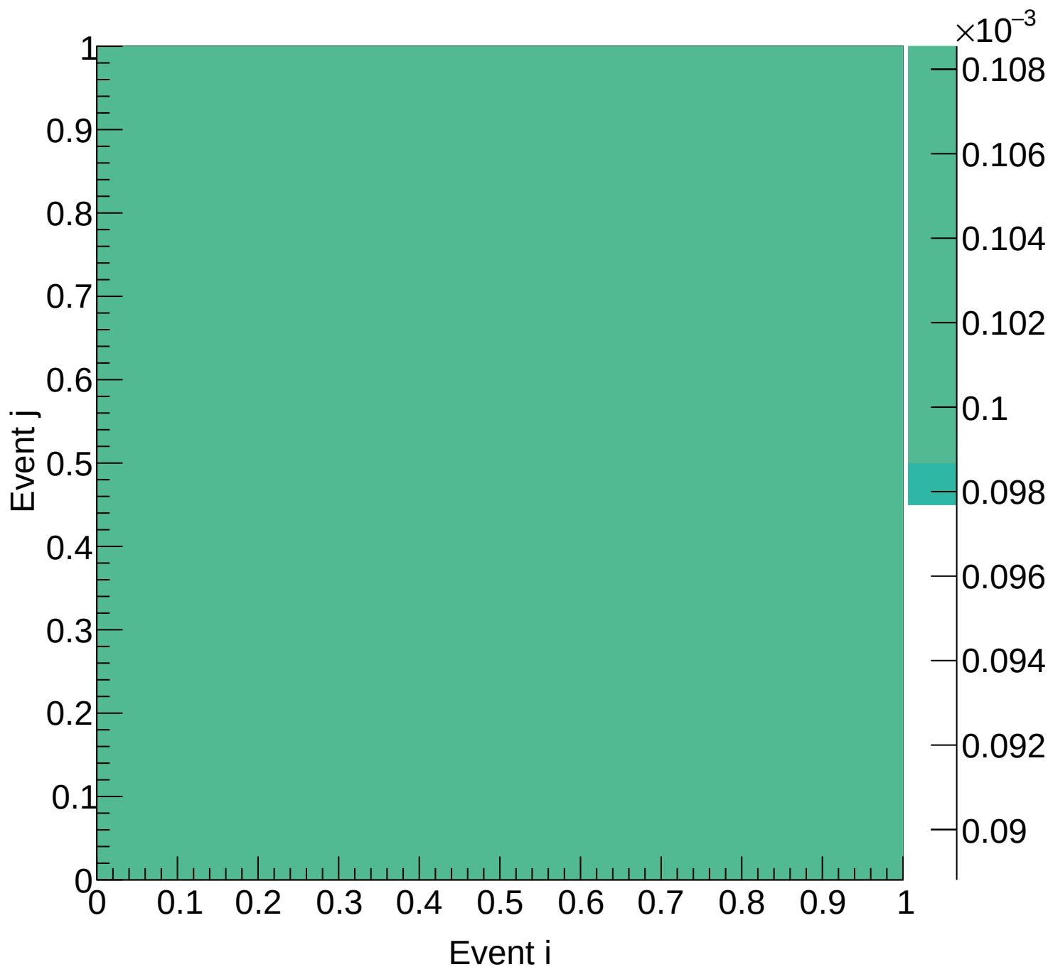
Flask (mix) Covariance | M: [5.7, 6.0) xF: [0.25, 0.30)
