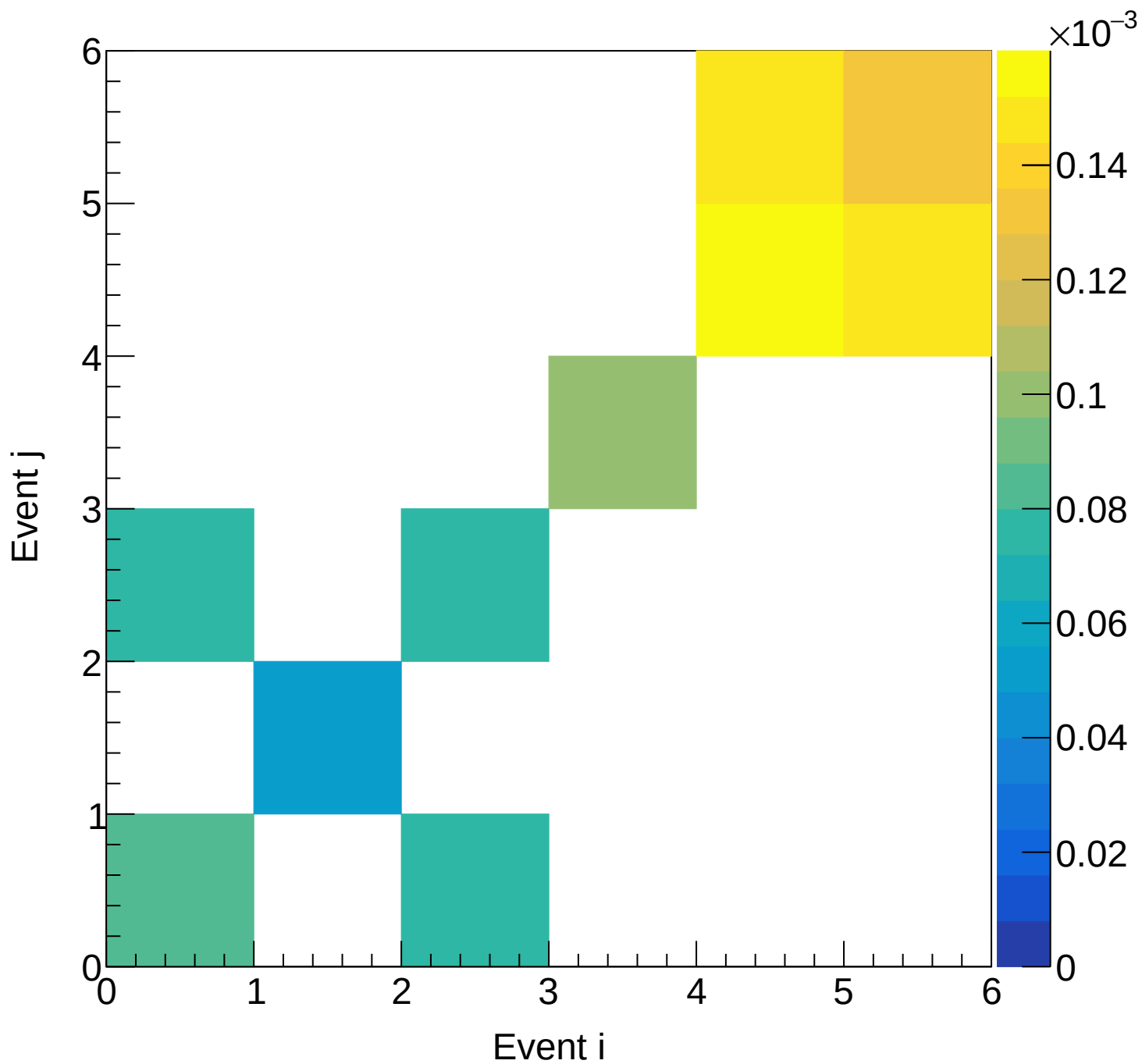
Flask (mix) Covariance | M: [3.9, 4.2) xF: [0.30, 0.35)
