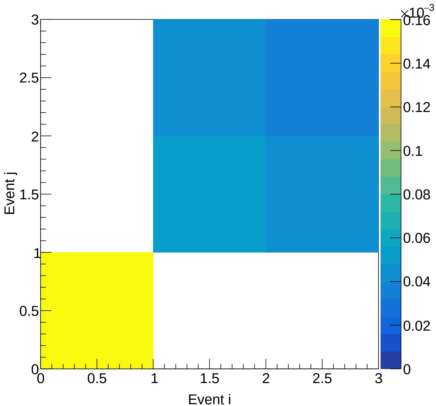
Flask (mix) Covariance | M: [4.2, 4.5) xF: [0.30, 0.35)
