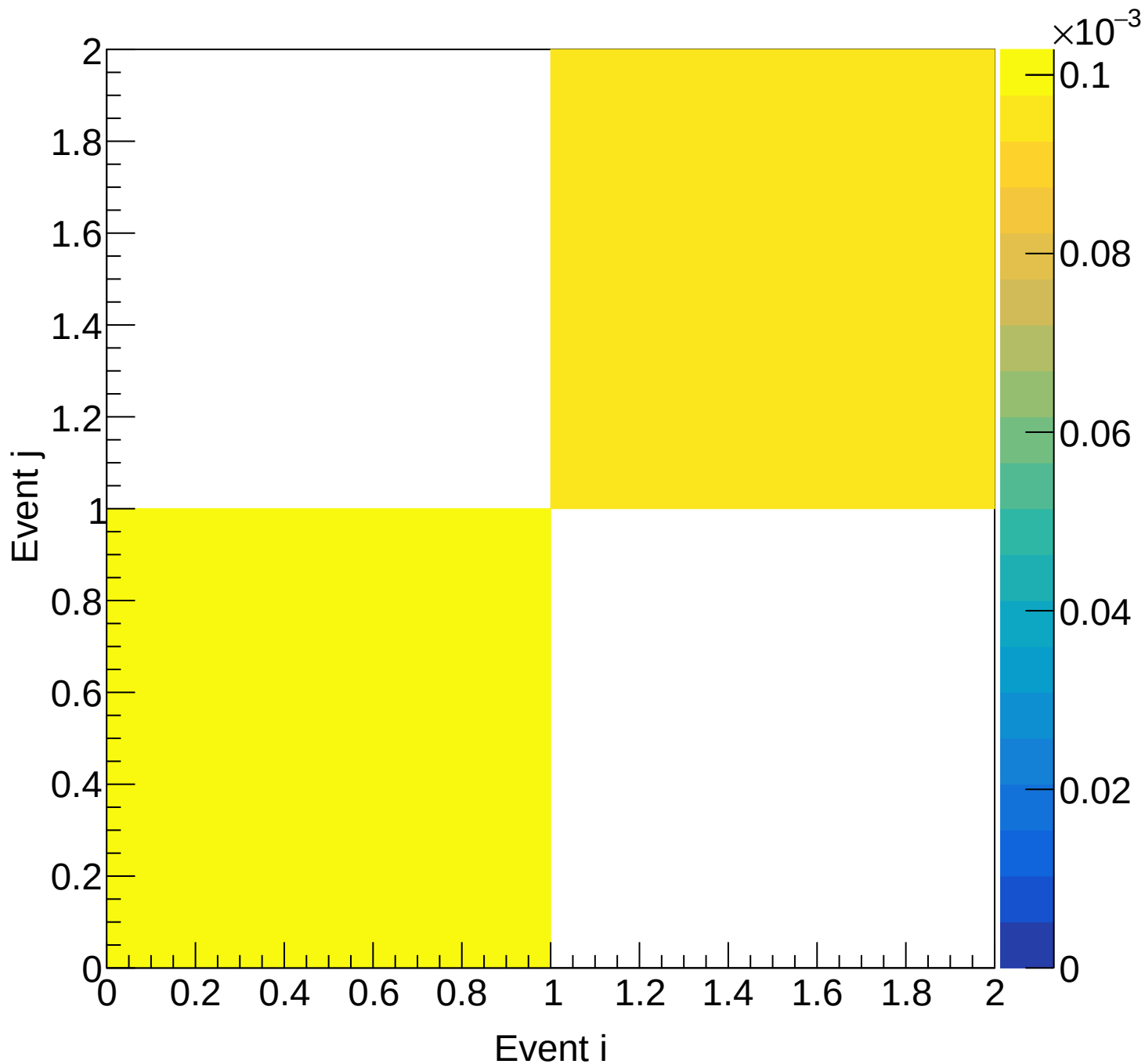
Flask (mix) Covariance | M: [4.8, 5.1) xF: [0.30, 0.35)
