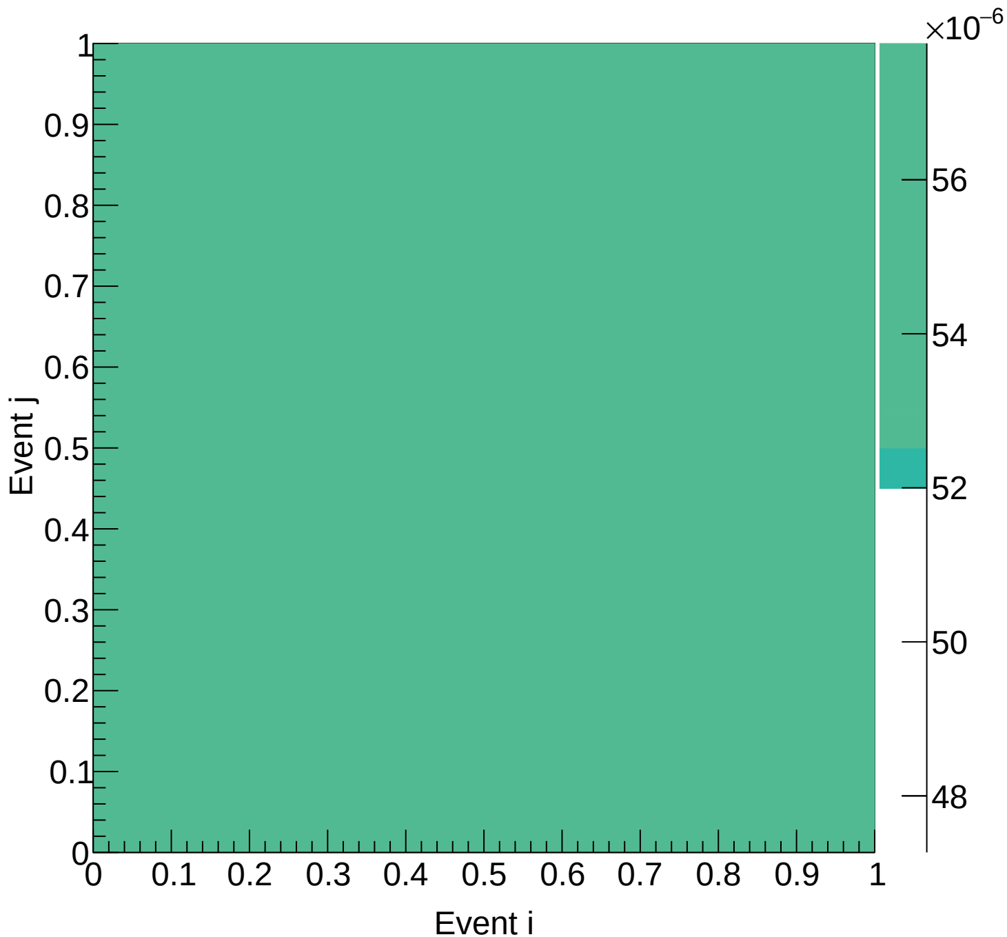
Flask (mix) Covariance | M: [5.1, 5.4) xF: [0.30, 0.35)
