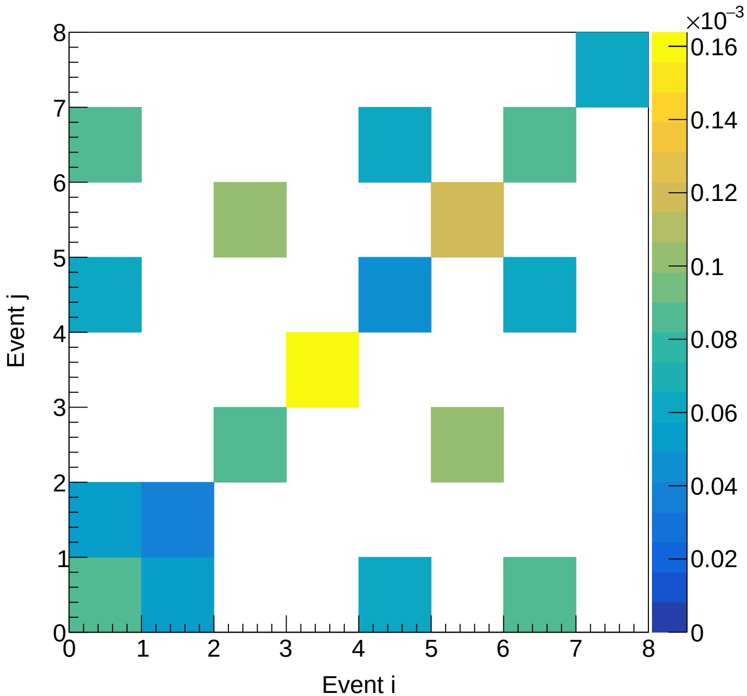
Flask (mix) Covariance | M: [3.9, 4.2) xF: [0.35, 0.40)
