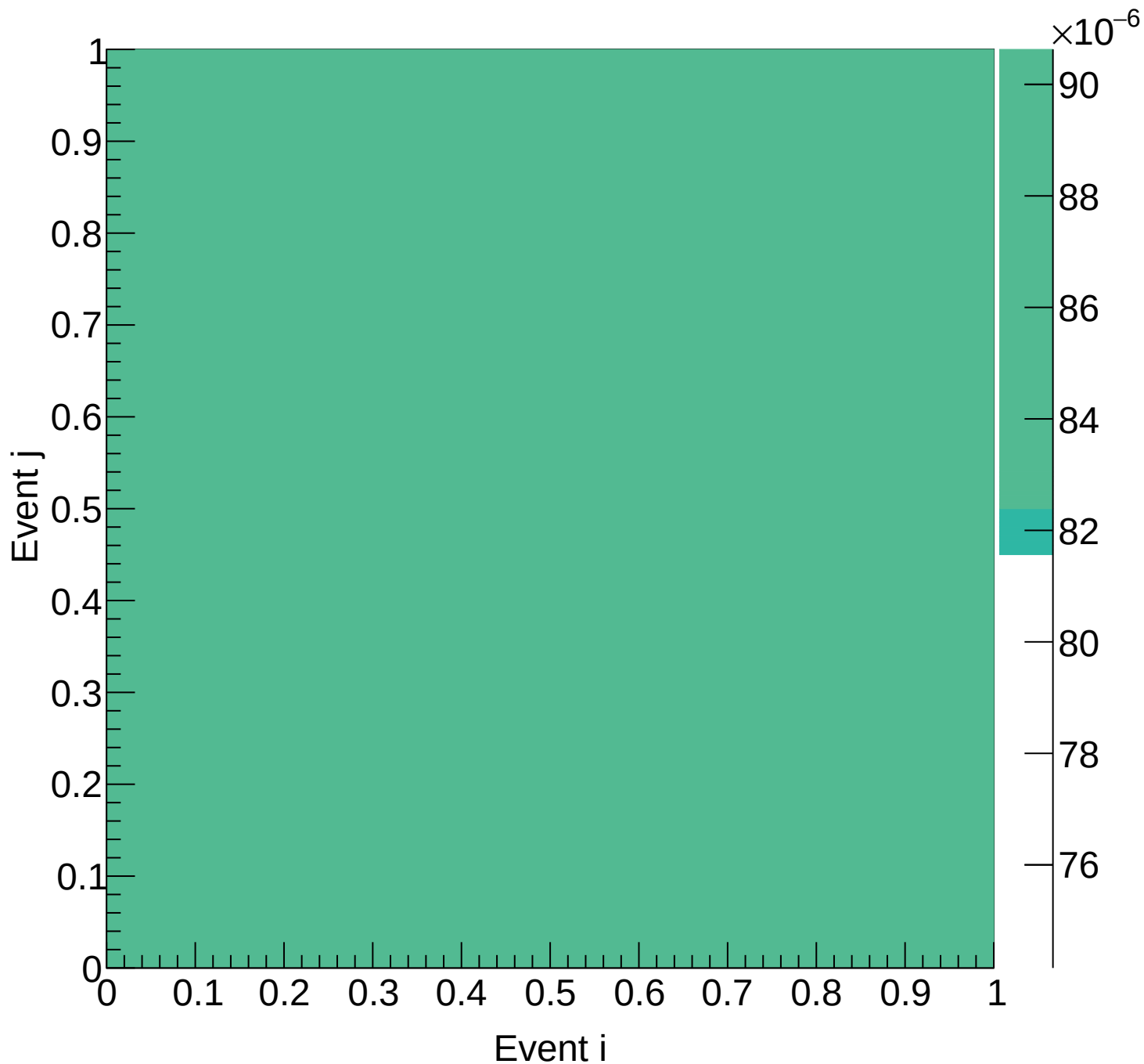
Flask (mix) Covariance | M: [5.1, 5.4) xF: [0.40, 0.45)
