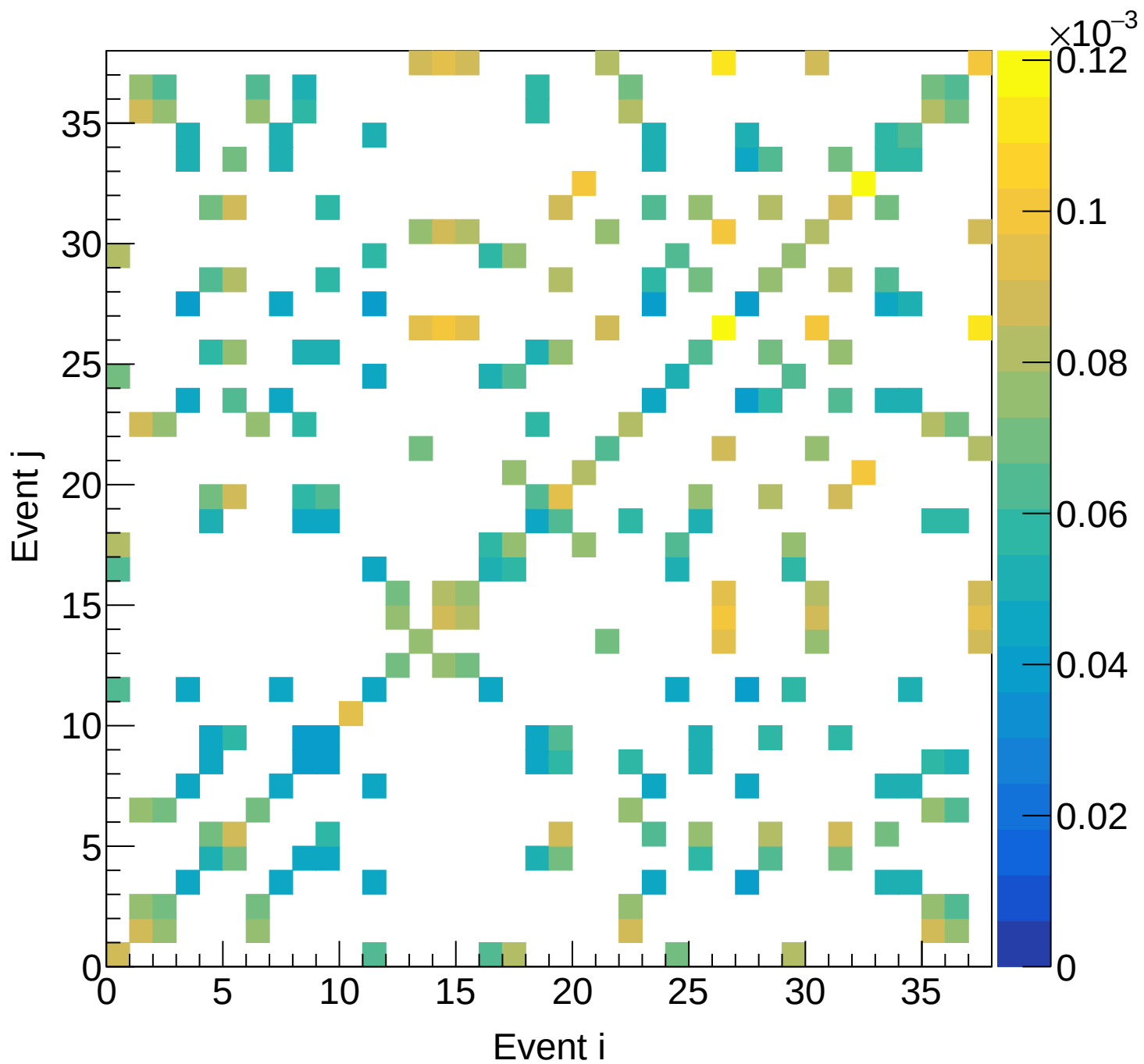
Flask (total) Covariance | M: [3.9, 4.2) xF: [0.45, 0.50)
