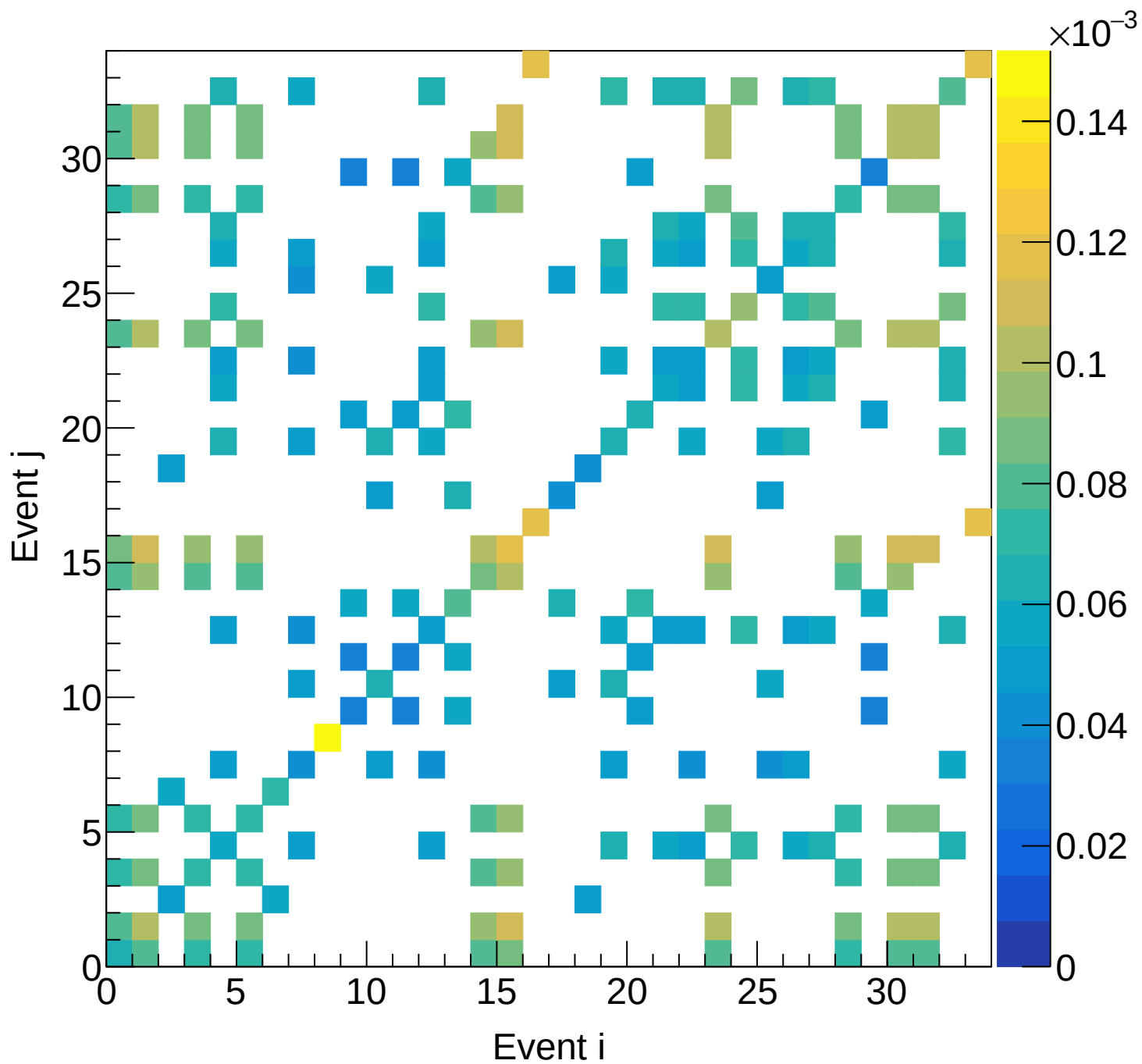
Flask (total) Covariance | M: [4.2, 4.5) xF: [0.45, 0.50)
