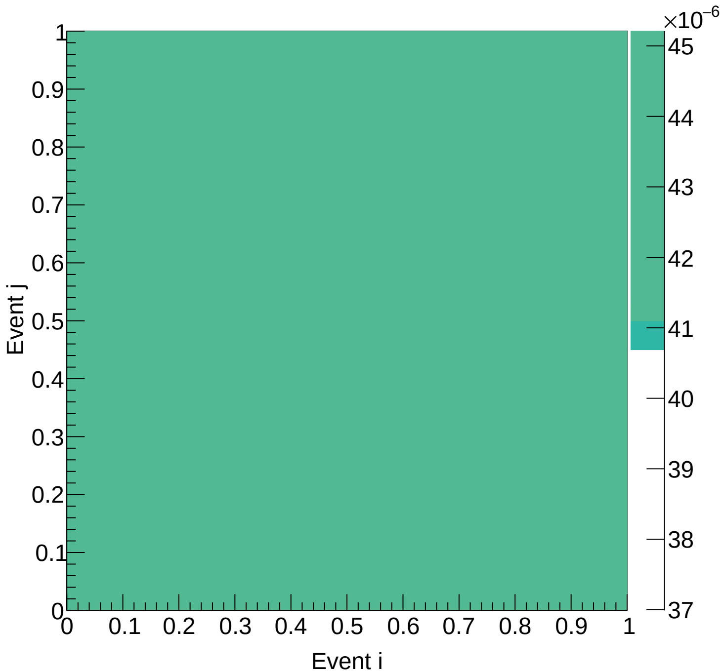
Flask (total) Covariance | M: [6.0, 6.3) xF: [0.45, 0.50)
