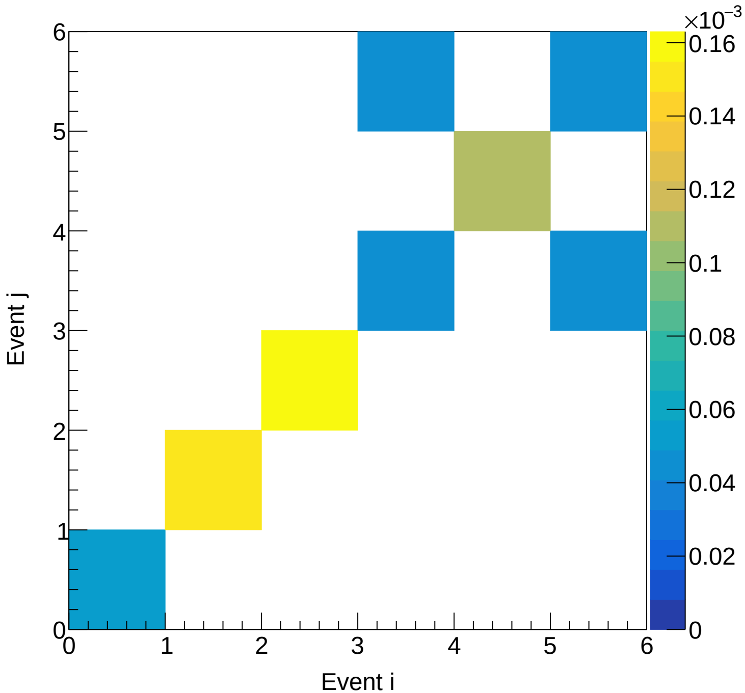
Flask (total) Covariance | M: [4.5, 4.8) xF: [0.55, 0.60)
