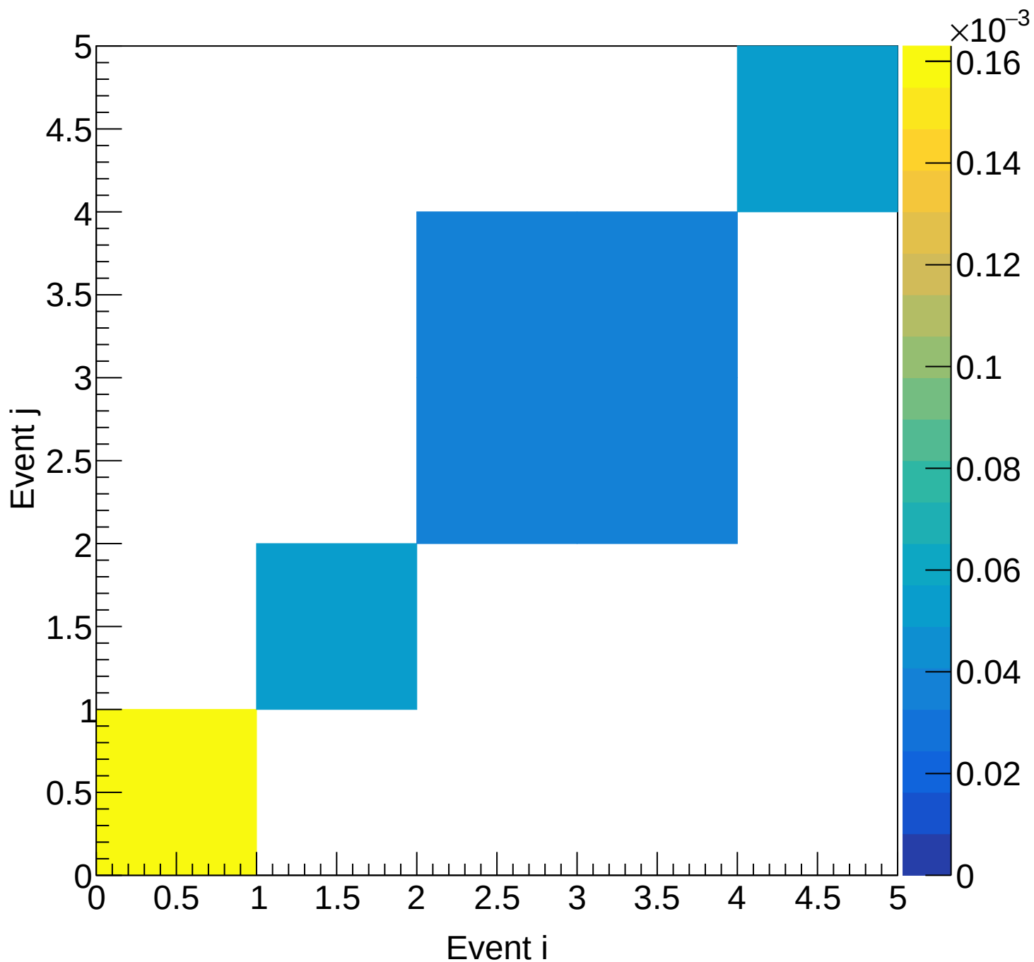
Flask (total) Covariance | M: [4.8, 5.1) xF: [0.55, 0.60)
