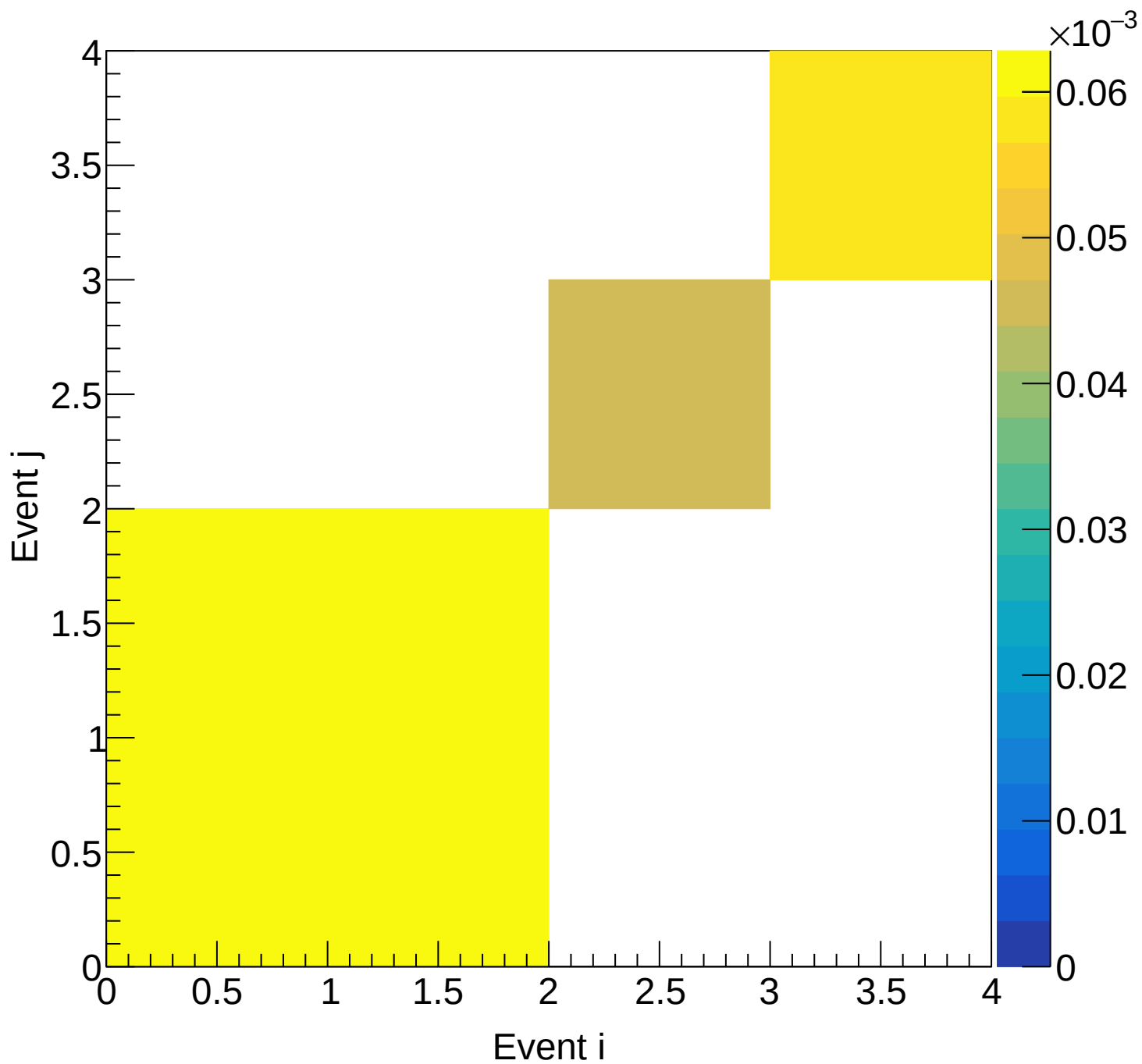
Flask (total) Covariance | M: [6.0, 6.3) xF: [0.55, 0.60)
