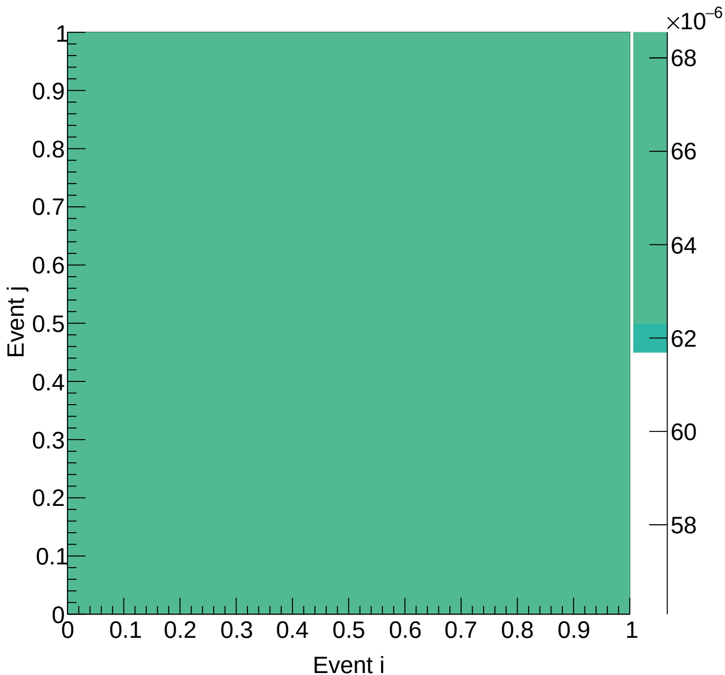
Flask (total) Covariance | M: [6.3, 6.6) xF: [0.55, 0.60)
