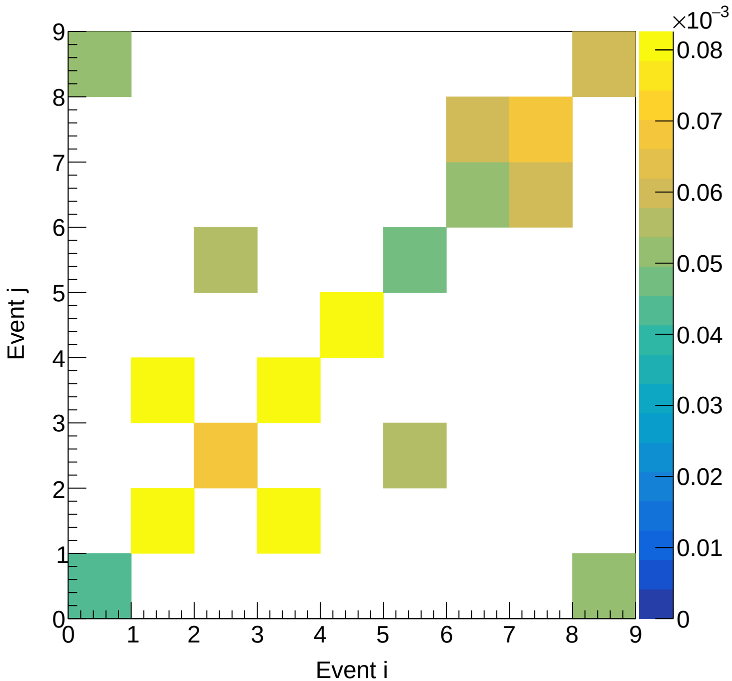
Flask (total) Covariance | M: [4.5, 4.8) xF: [0.60, 0.65)
