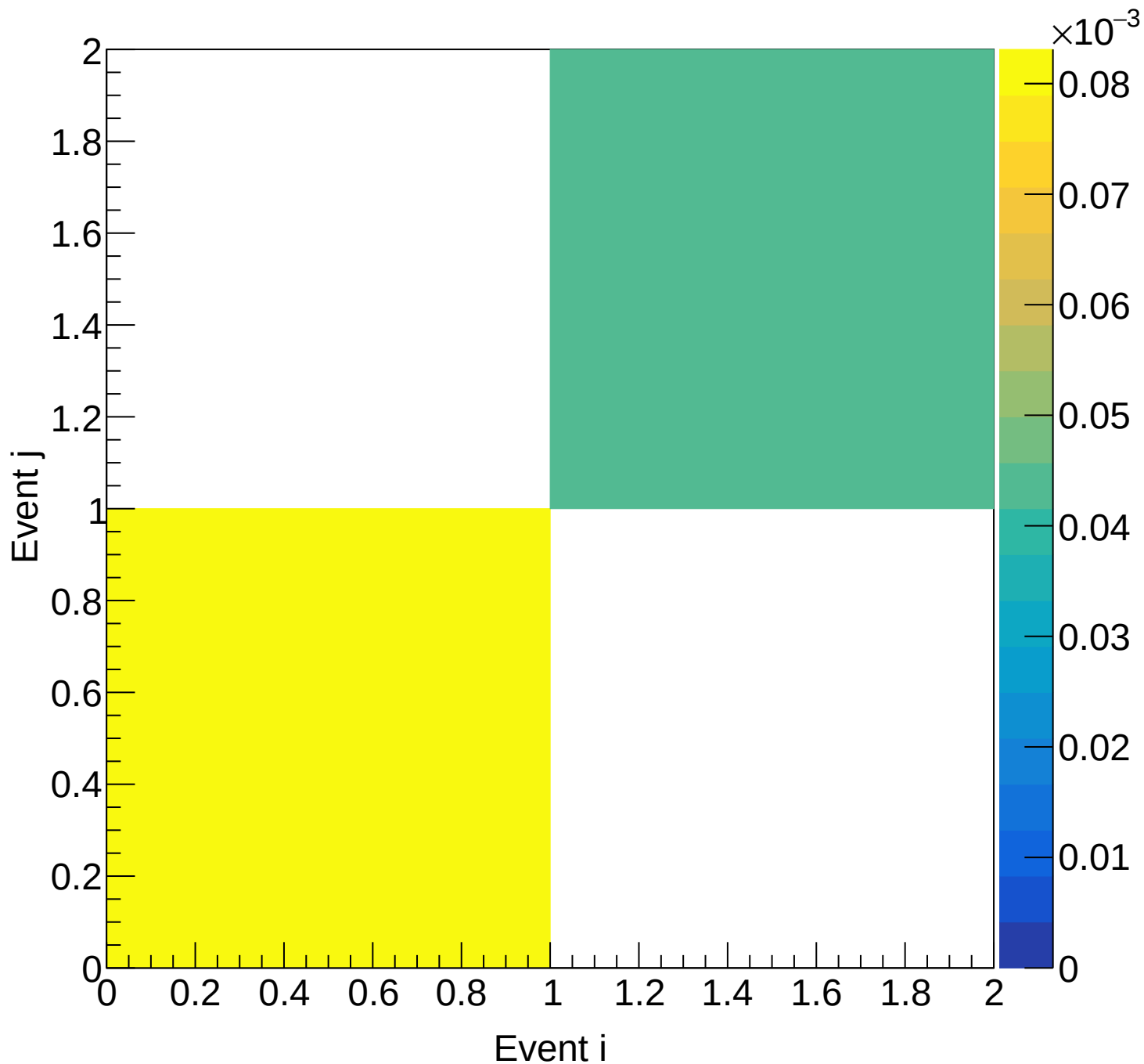
Flask (total) Covariance | M: [5.4, 5.7) xF: [0.60, 0.65)
