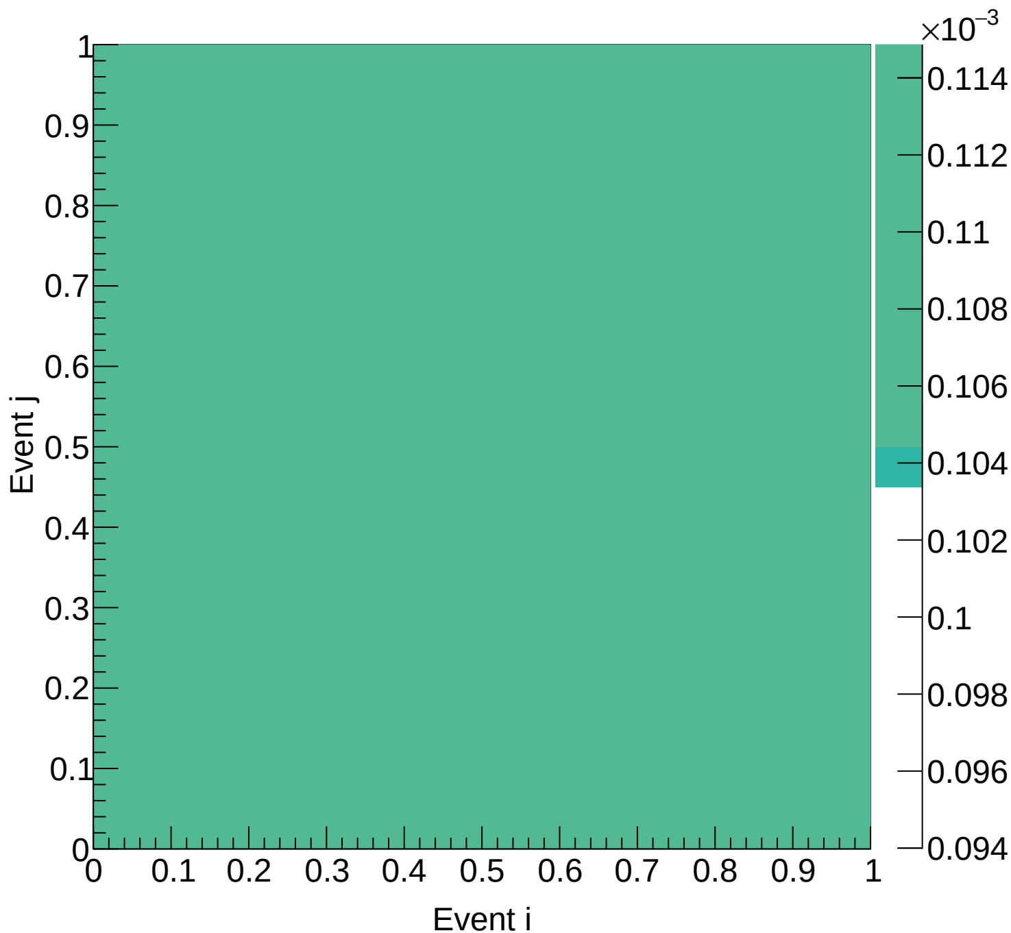
Flask (total) Covariance | M: [6.6, 6.9) xF: [0.60, 0.65)
