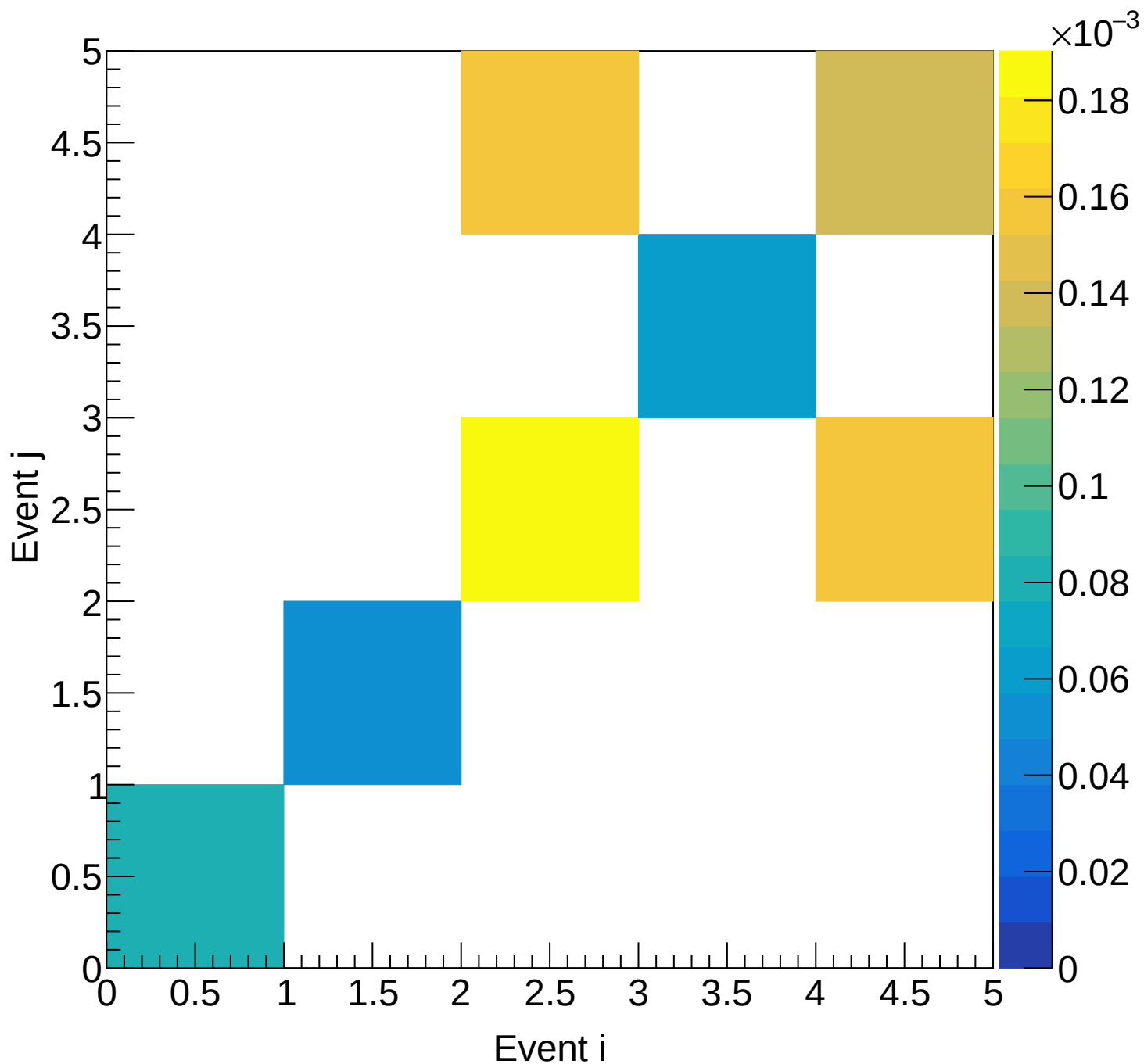
Flask (total) Covariance | M: [5.1, 5.4) xF: [0.65, 0.70)
