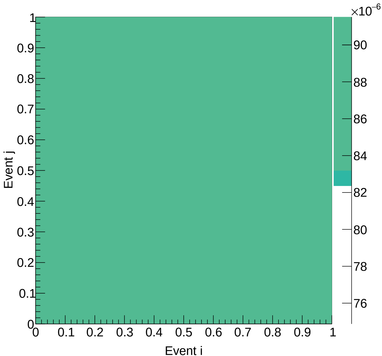
Flask (total) Covariance | M: [6.0, 6.3) xF: [0.65, 0.70)
