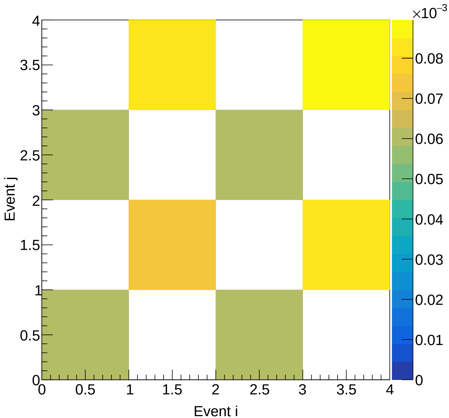
Flask (total) Covariance | M: [4.2, 4.5) xF: [0.70, 0.75)
