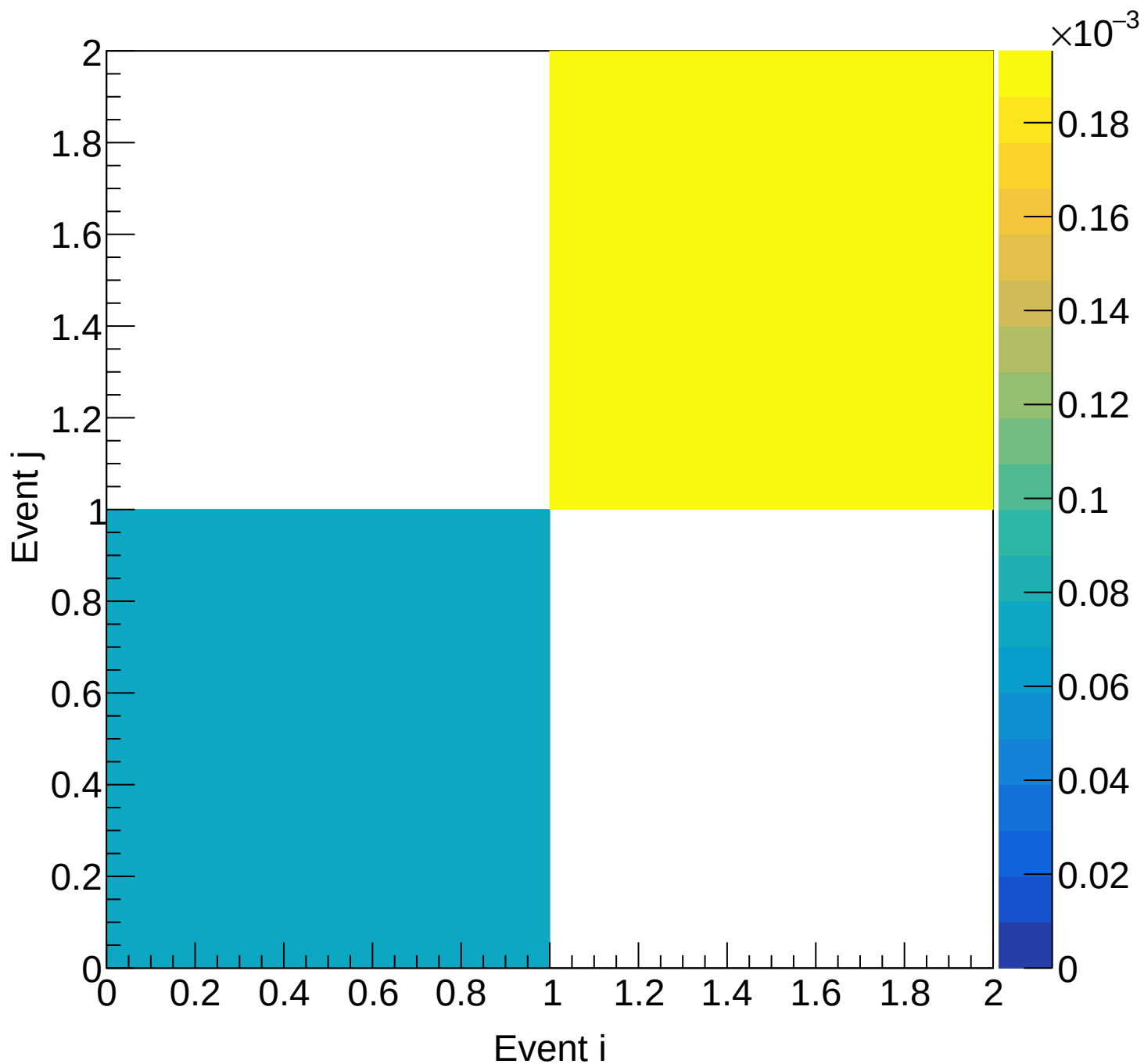
Flask (total) Covariance | M: [4.8, 5.1) xF: [0.70, 0.75)
