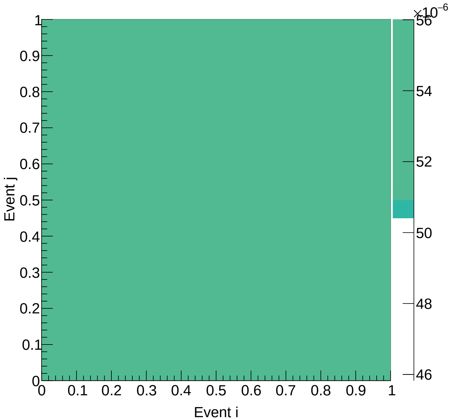
Flask (total) Covariance | M: [6.6, 6.9) xF: [0.70, 0.75)
