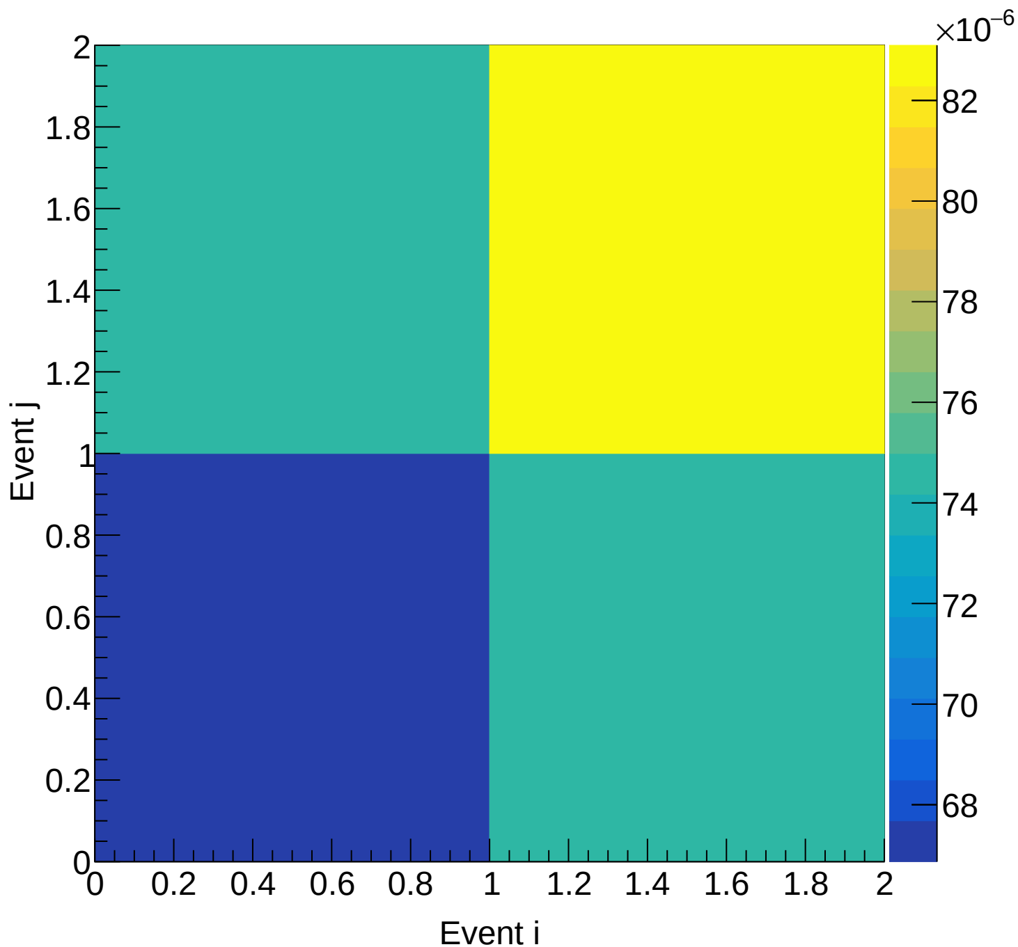
Flask (total) Covariance | M: [4.2, 4.5) xF: [0.75, 0.80)
