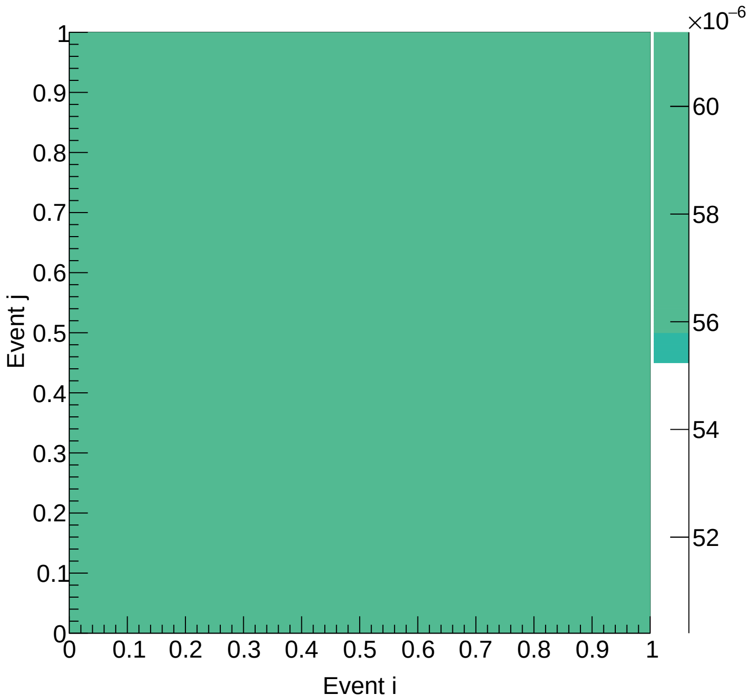
Flask (total) Covariance | M: [5.4, 5.7) xF: [0.75, 0.80)
